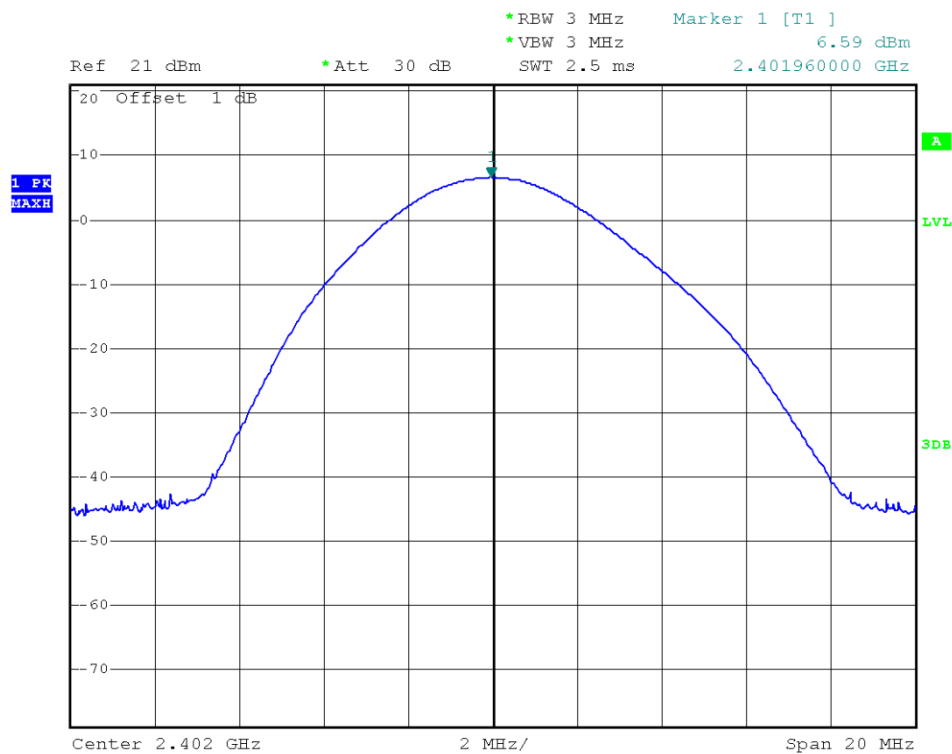
Plot C1:8-DPSK
