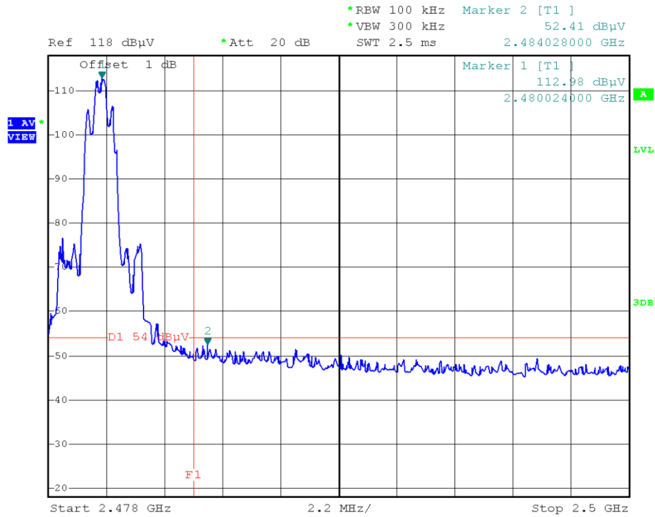
(Plot D2: Channel = 78 AVERAGE @ \pi/4 -DQPSK)
