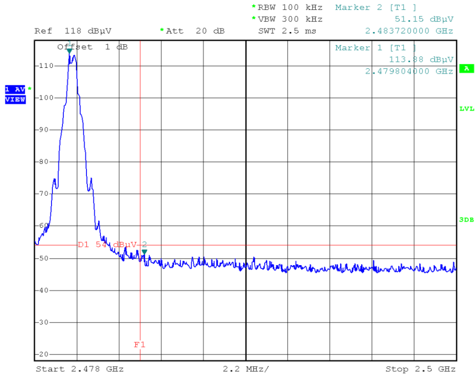
(Plot B2: Channel = 78 AVERAGE @ GFSK)
