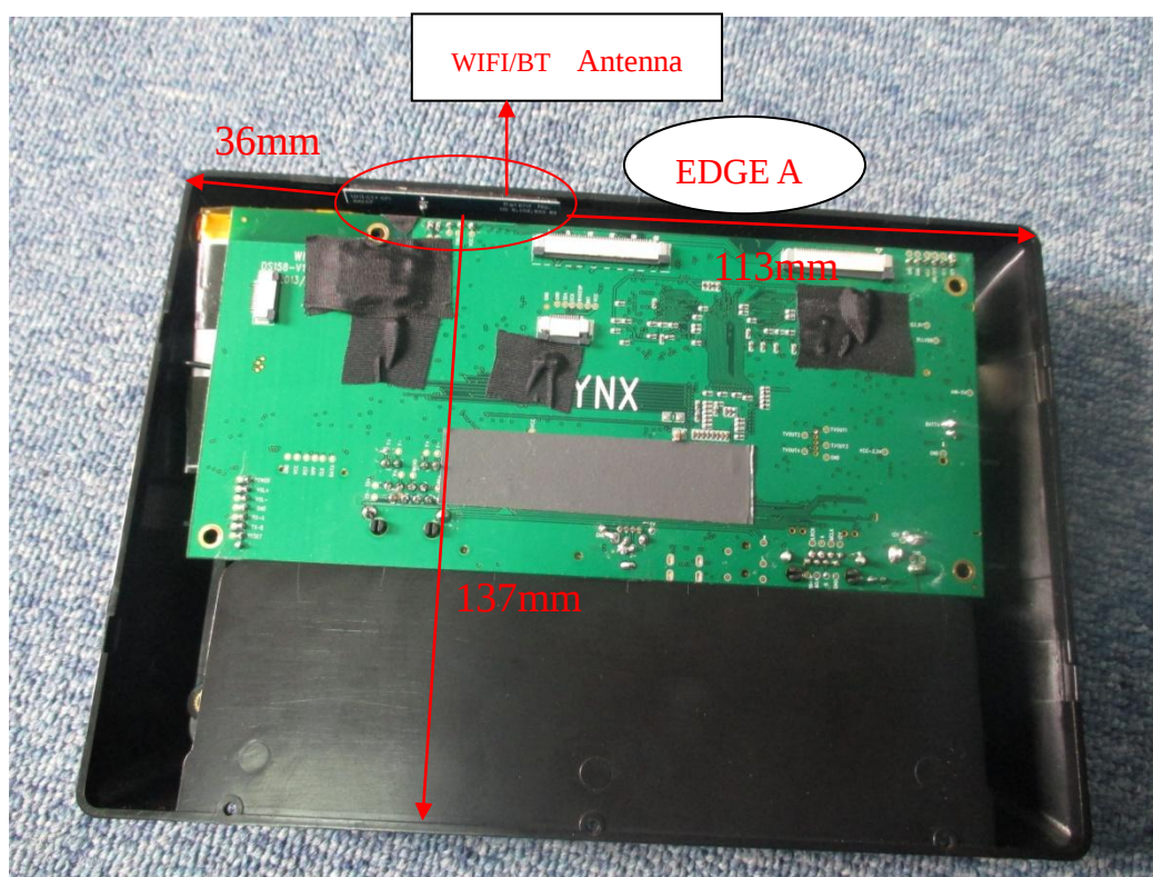
Fig. 3 Position of antenna
