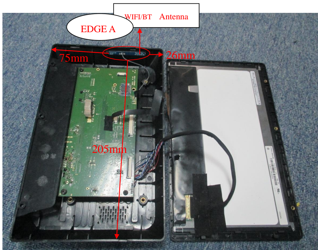
Fig. 3 Position of antenna
