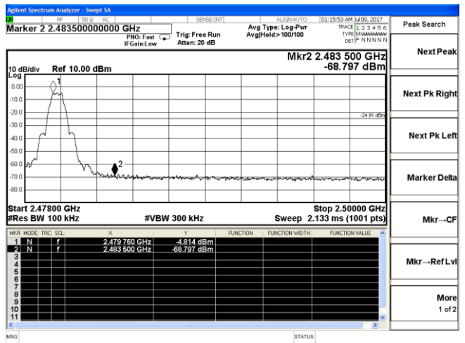
Channel 39 / 2480 MHz
