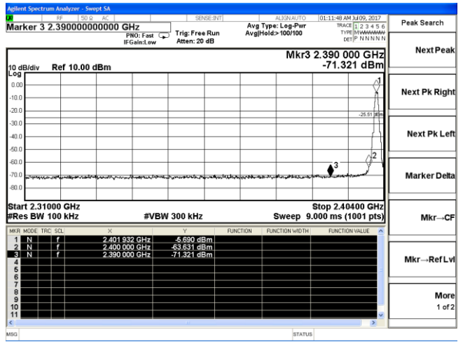
Channel 0 / 2402 MHz
