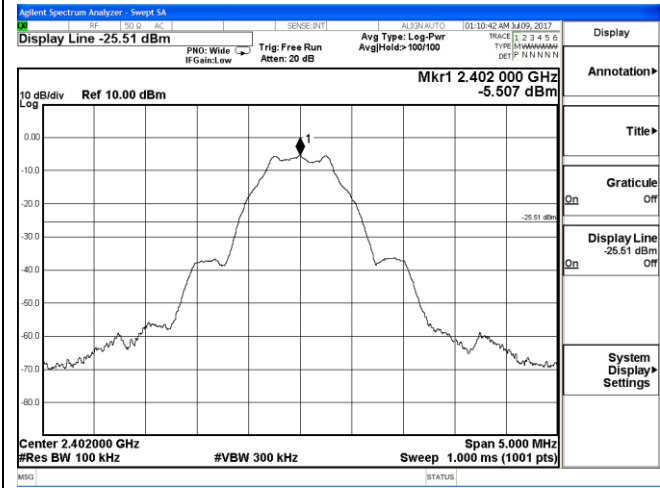
2399.5 – 2404.5 MHz
