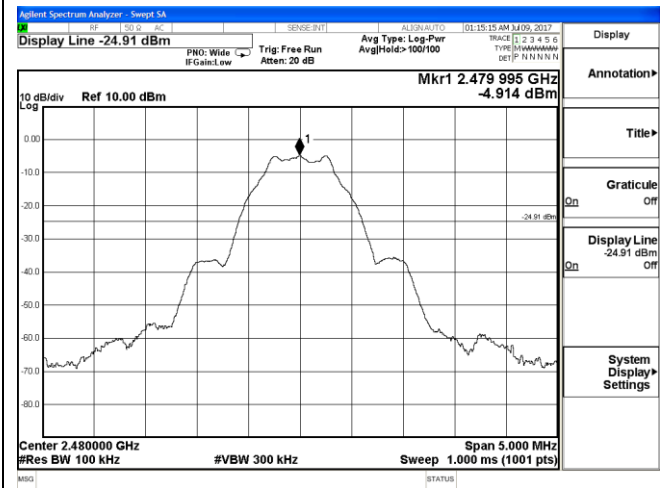
2477.5 – 2482.5 MHz
