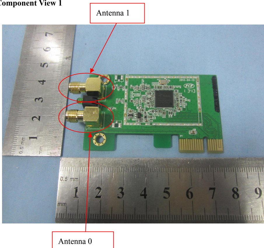
Solder Board-Component View 1
