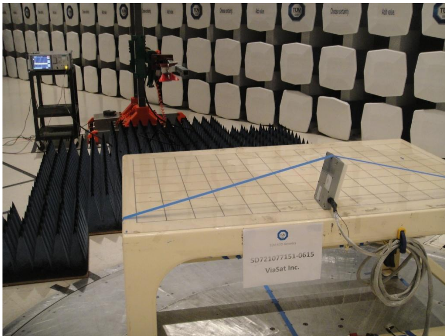
Setup for WiFi Radiated Emission Above 1GHz Front and Back
