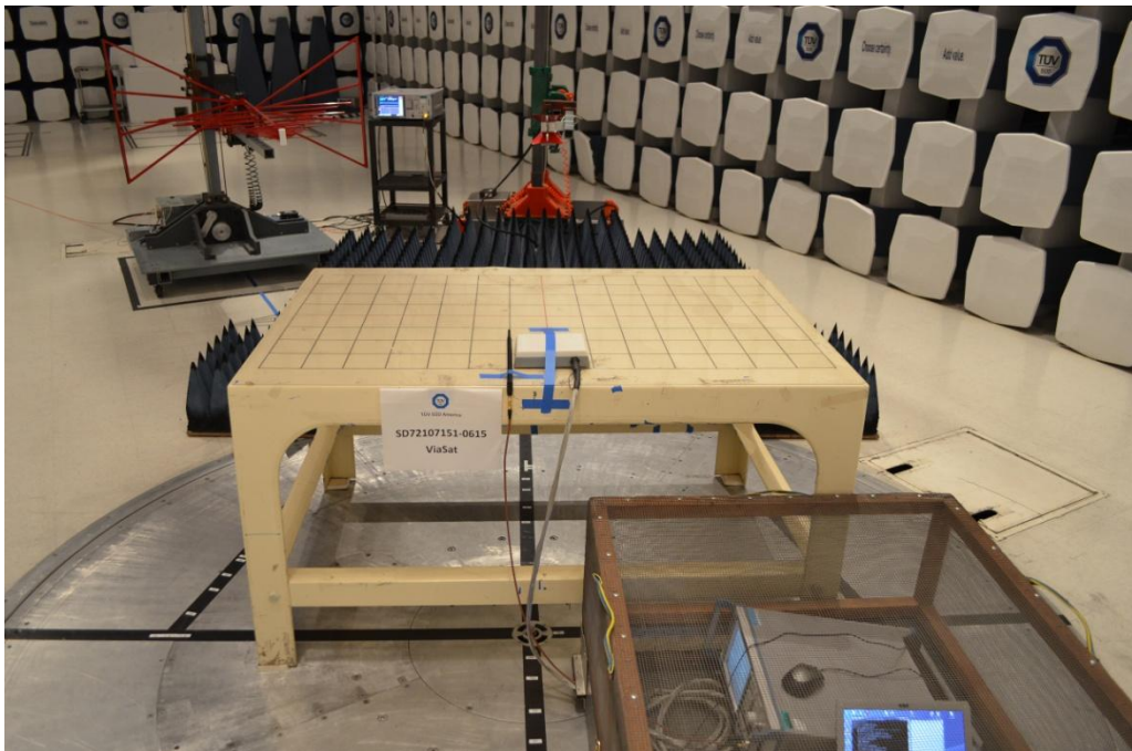
Setup for Bluetooth Radiated Emission Above 1GHz Front and Back
