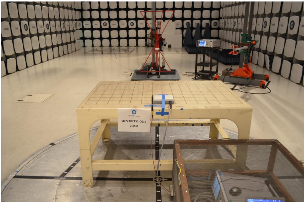
Setup for Bluetooth Radiated Emission Below 1GHz Front and Back
