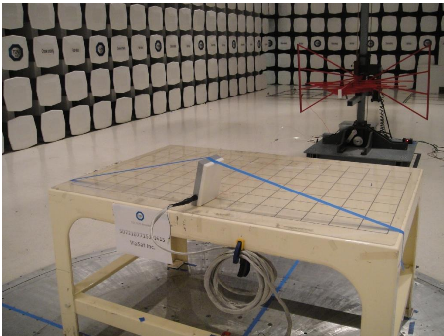
Setup for WiFi Radiated Emission Below 1GHz Front and Back
