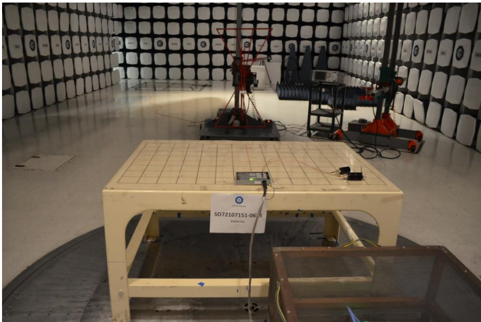
Setup for Satellite test Radiated Emission Below 1GHz Front and Back
