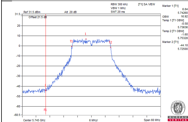
802.11a_Chain 2 / CH149
