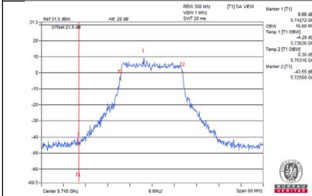
802.11a_Chain 6 / CH149
