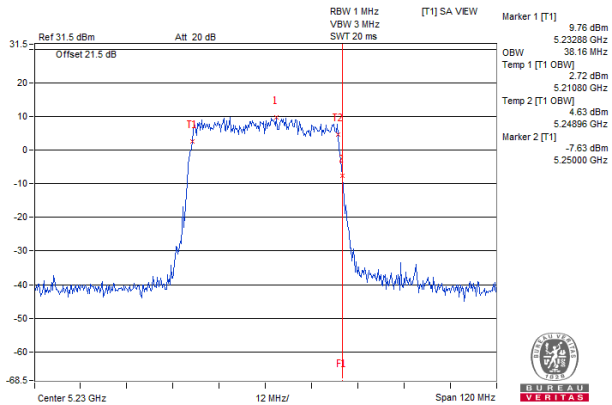
802.11ax (HE40) Chain 6 / CH46
