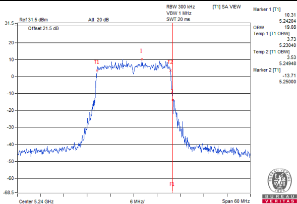
802.11ax (HE20) Chain 4 / CH48
