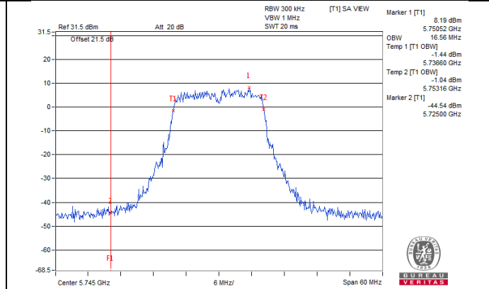
802.11a_Chain 5 / CH149
