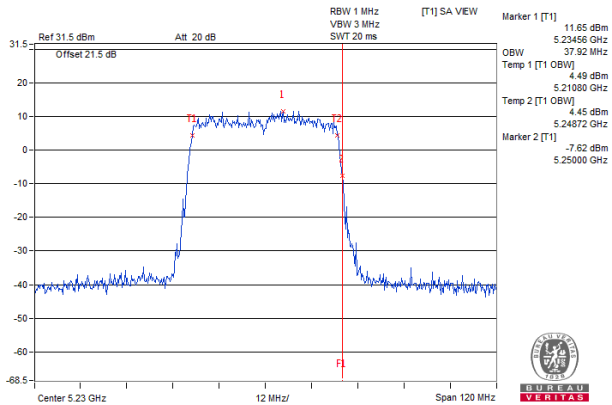
802.11ax (HE40) Chain 4 / CH46
