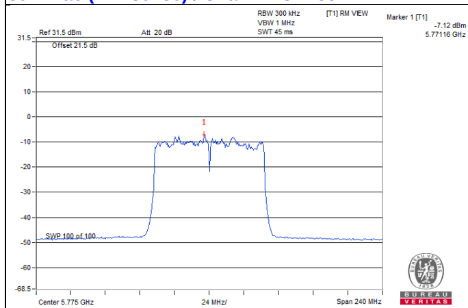
802.11ac (VHT80+80) / Chain 7: CH155
