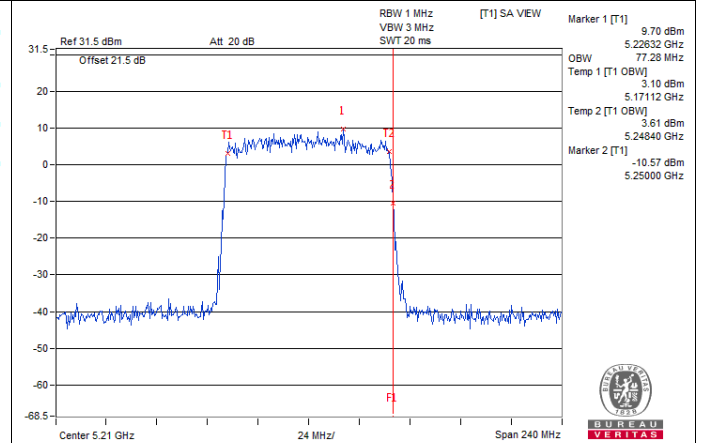
802.11ax (HE80+80) / Chain 3 : CH42
