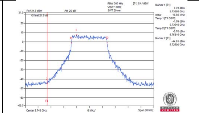
802.11a_Chain 7 / CH149
