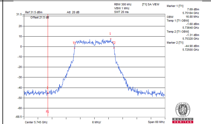
802.11a_Chain 3 / CH149
