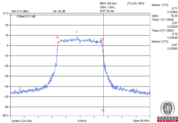
802.11ax (HE20) Chain 2 / CH48
