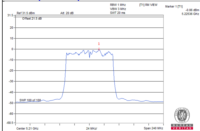
802.11ac (VHT80+80) / Chain 0 : CH42
