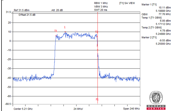
802.11ax (HE80+80) / Chain 2 : CH42
