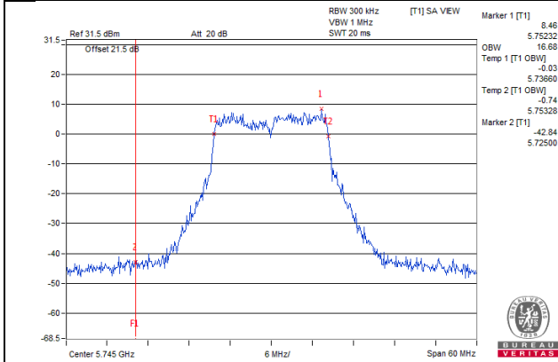
802.11a_Chain 4 / CH149
