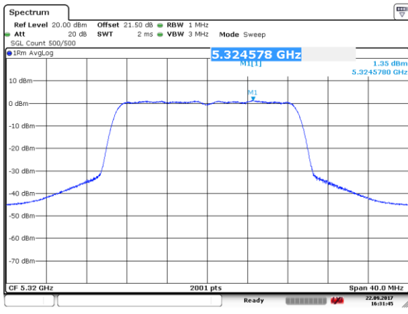
Channel 64 (5320MHz)
