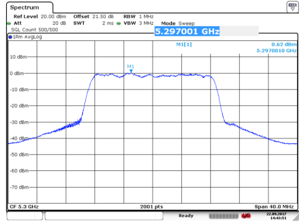
Channel 60 (5300MHz)
