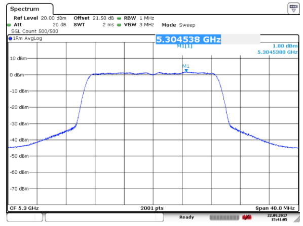
Channel 60 (5300MHz)
