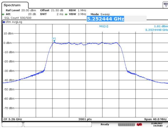
Channel 52 (5260MHz)
