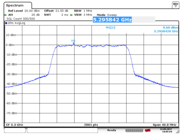
Channel 60 (5300MHz)
