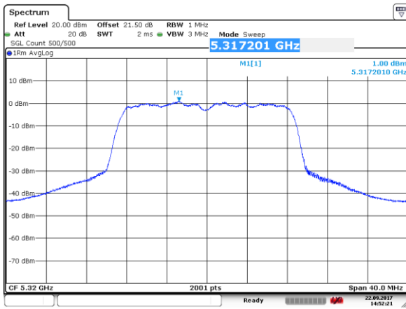
Channel 64 (5320MHz)
