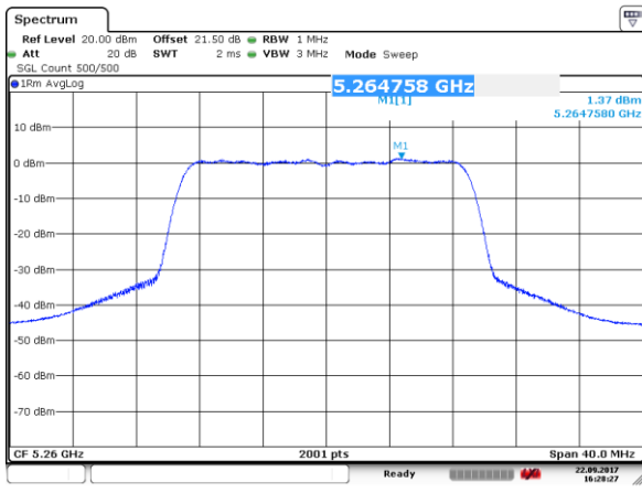
Channel 52 (5260MHz)
