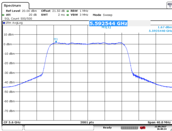
Channel 120 (5600MHz)
