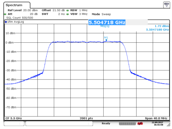
Channel 100 (5500MHz)
