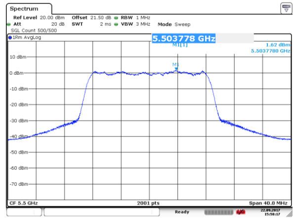
Channel 100 (5500MHz)
