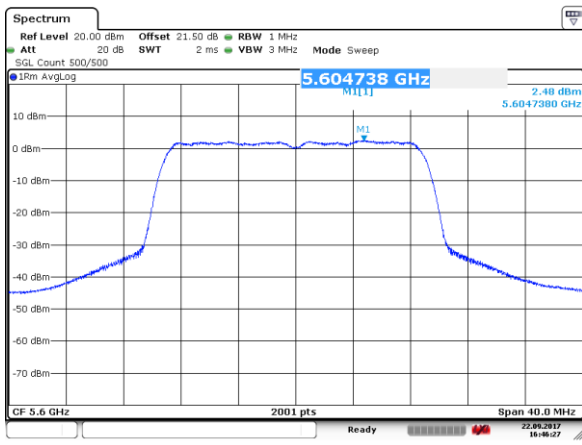
Channel 120 (5600MHz)
