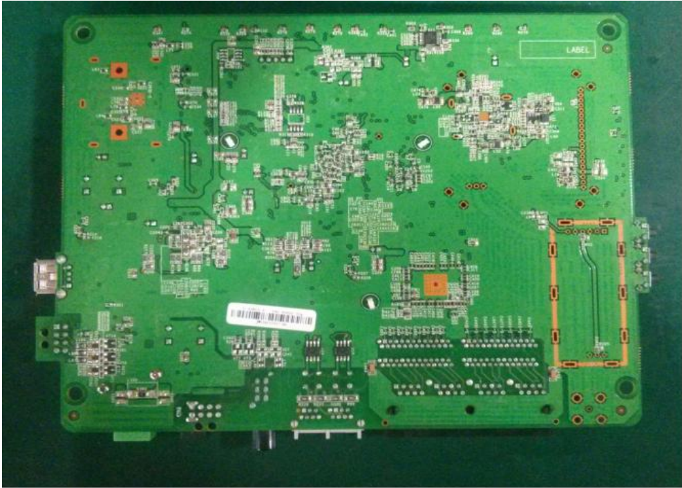
(4) EUT Photo (TO73G)
