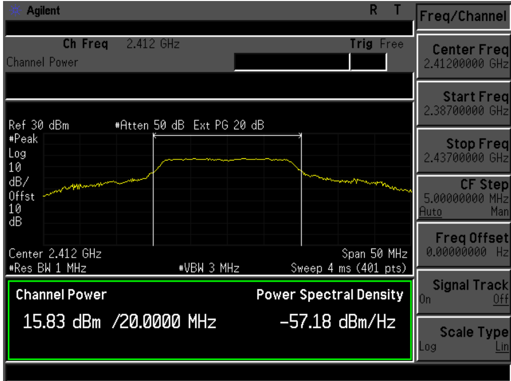
Channel 01 (2412MHz)
