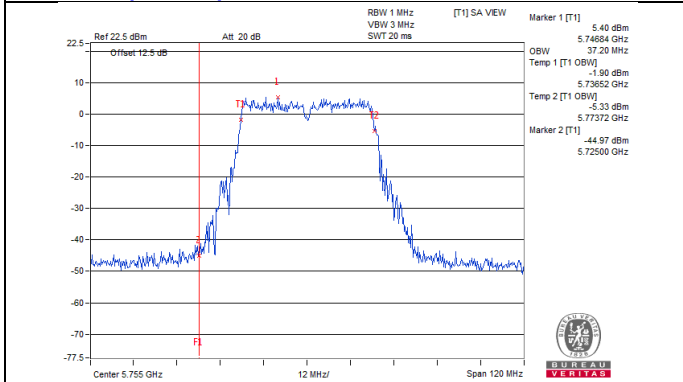
802.11ac (VHT40)_Chain 6 / CH151
