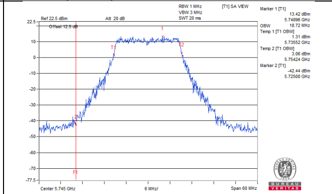
802.11ac (VHT20)_Chain 3 / CH149
