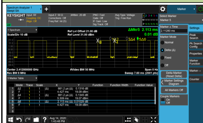
802.11n-HT20 (T = 16.200ms)
