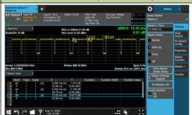
802.11n-HT40 (T = 10.700ms)
