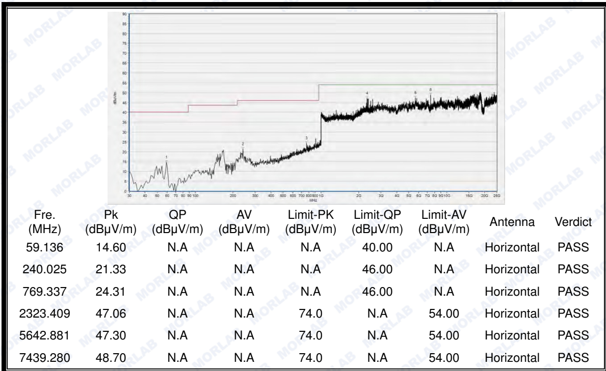
(30MHz to 25GHz, Antenna Horizontal @ π/4-DQPSK, channel 78)
