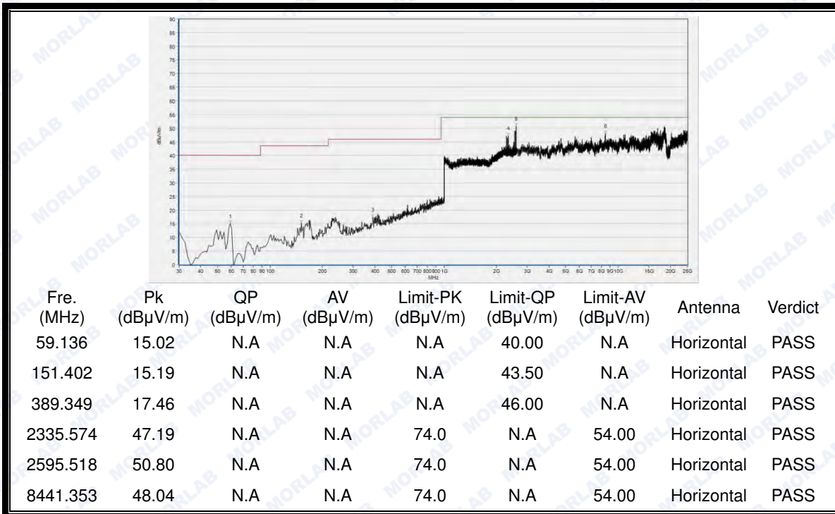
(30MHz to 25GHz, Antenna Horizontal @ π/4-DQPSK, channel 39)
