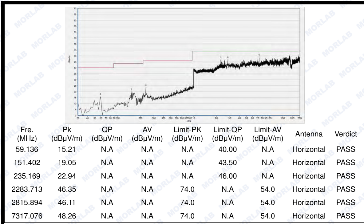
(30MHz to 25GHz, Antenna Horizontal @8-DPSK, channel 39)
