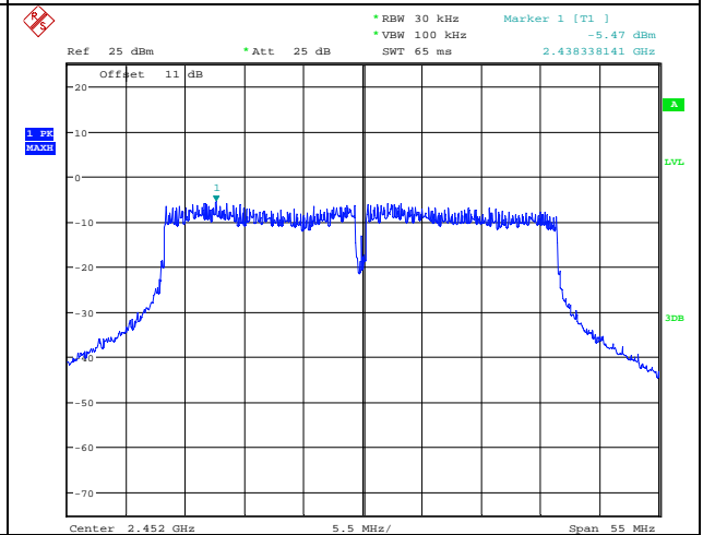
11n HT 40 CH9/Chain 1
