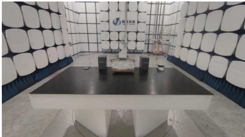
Radiated Emissions From 30M-1GHz
