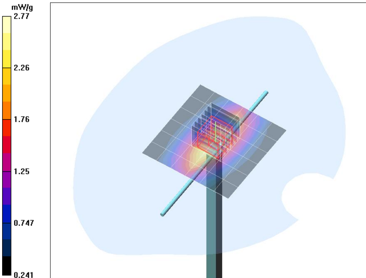
Fig. 4: Validation measurement 835 MHz Body (WCDMA V, July 04, 2014), coarse grid. Ambient Temperature: 21.8°C. Liquid Temperature: 21.2°C.
