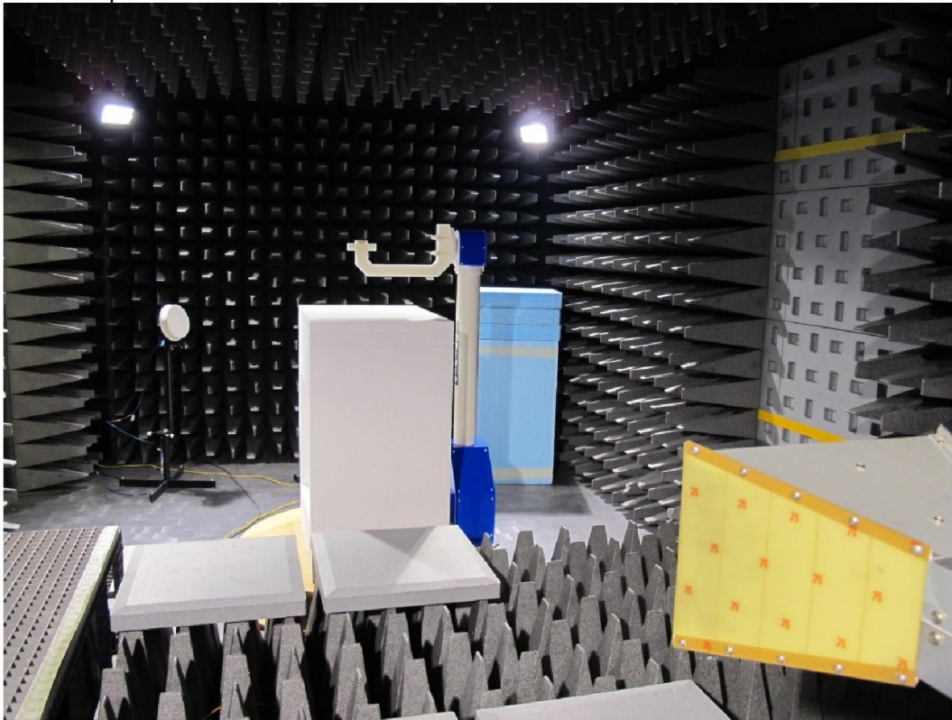
Test set up radiated emission 1GHz – 26.5 GHz
