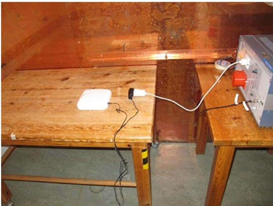
Test set up Conducted emission test 150 kHz – 30 MHz
