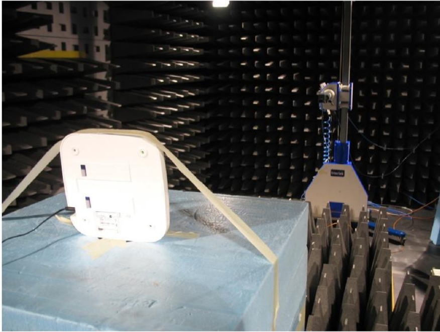
Test set up radiated emission > 18GHz
