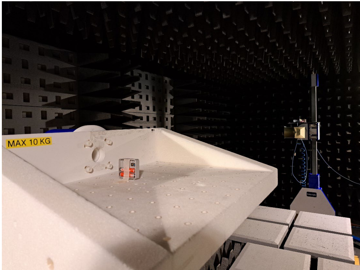
Photo of the test set-up for radiated emission 1 – 26.5 GHz
