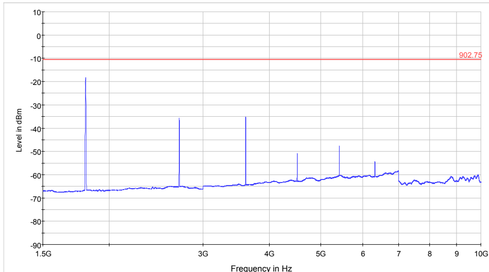
Average-MaxHold-AVG 902.75
