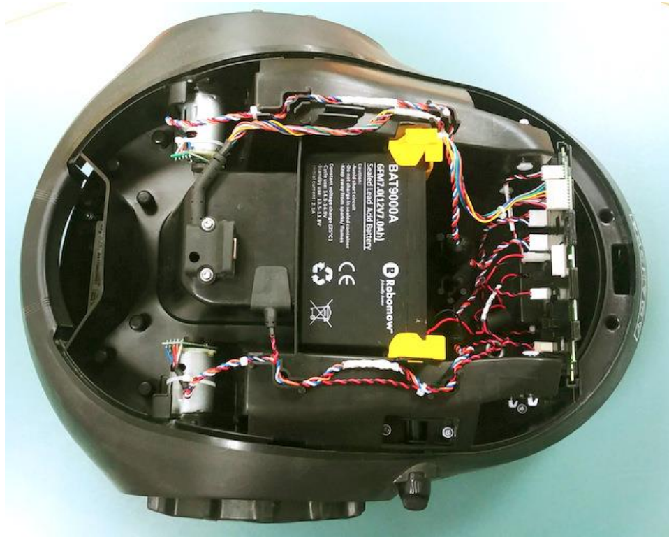
RX/XR1 host without the plastic cover. The plastic cover does not affect the location of any internal electronics or RF modules.
