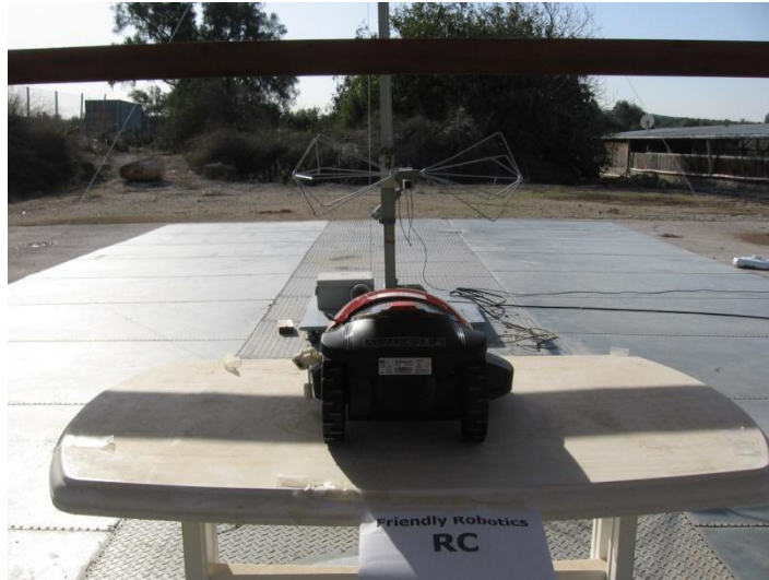
Radiated Emission Test RC
