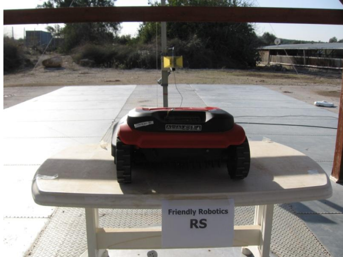
Radiated Emission Test RS
