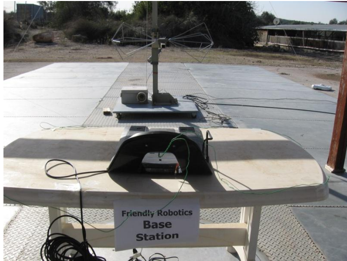
Radiated Emission Test Base Station
