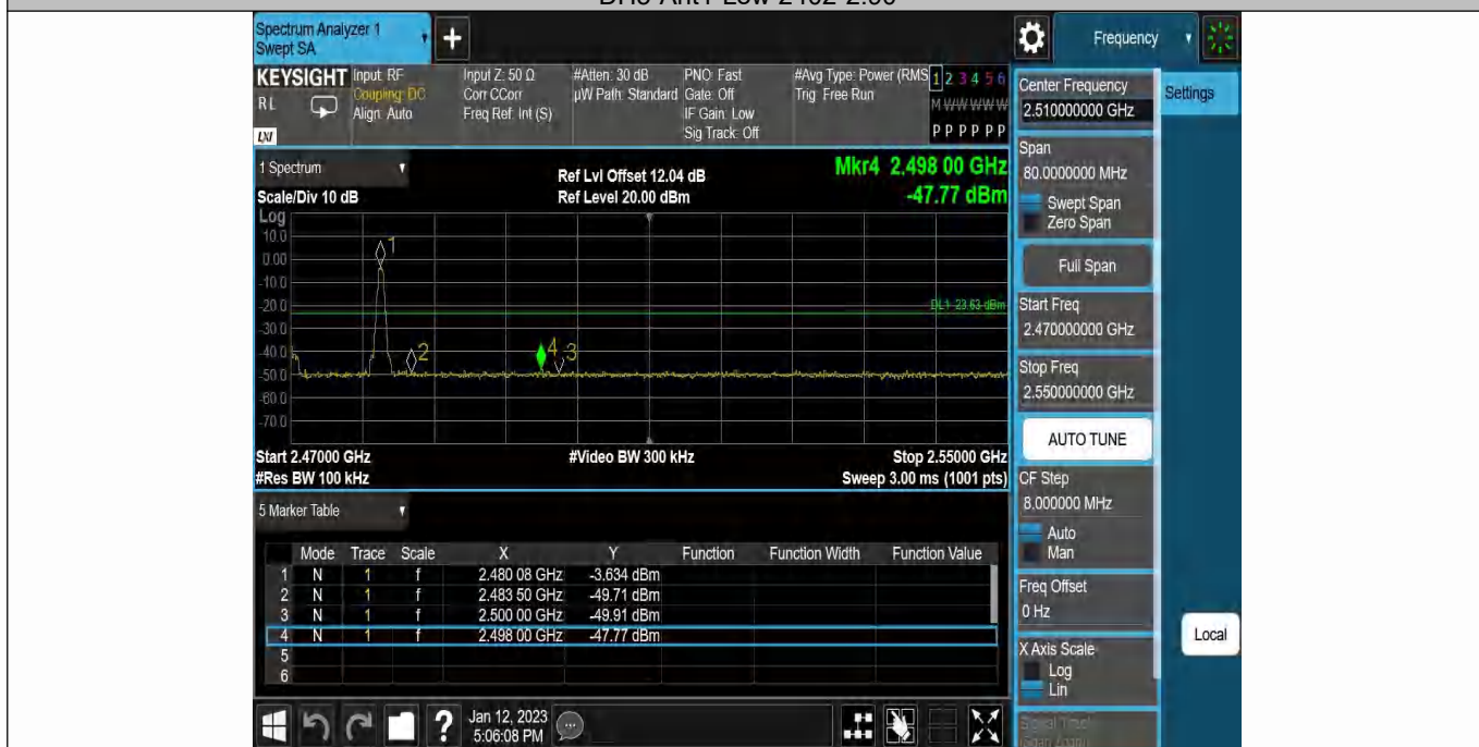
DH5-Ant1-High-2480--3.63
