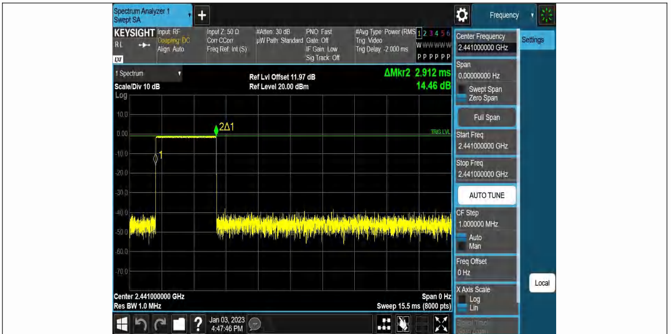
DH5-Ant1-Hop-2.912-106.67
