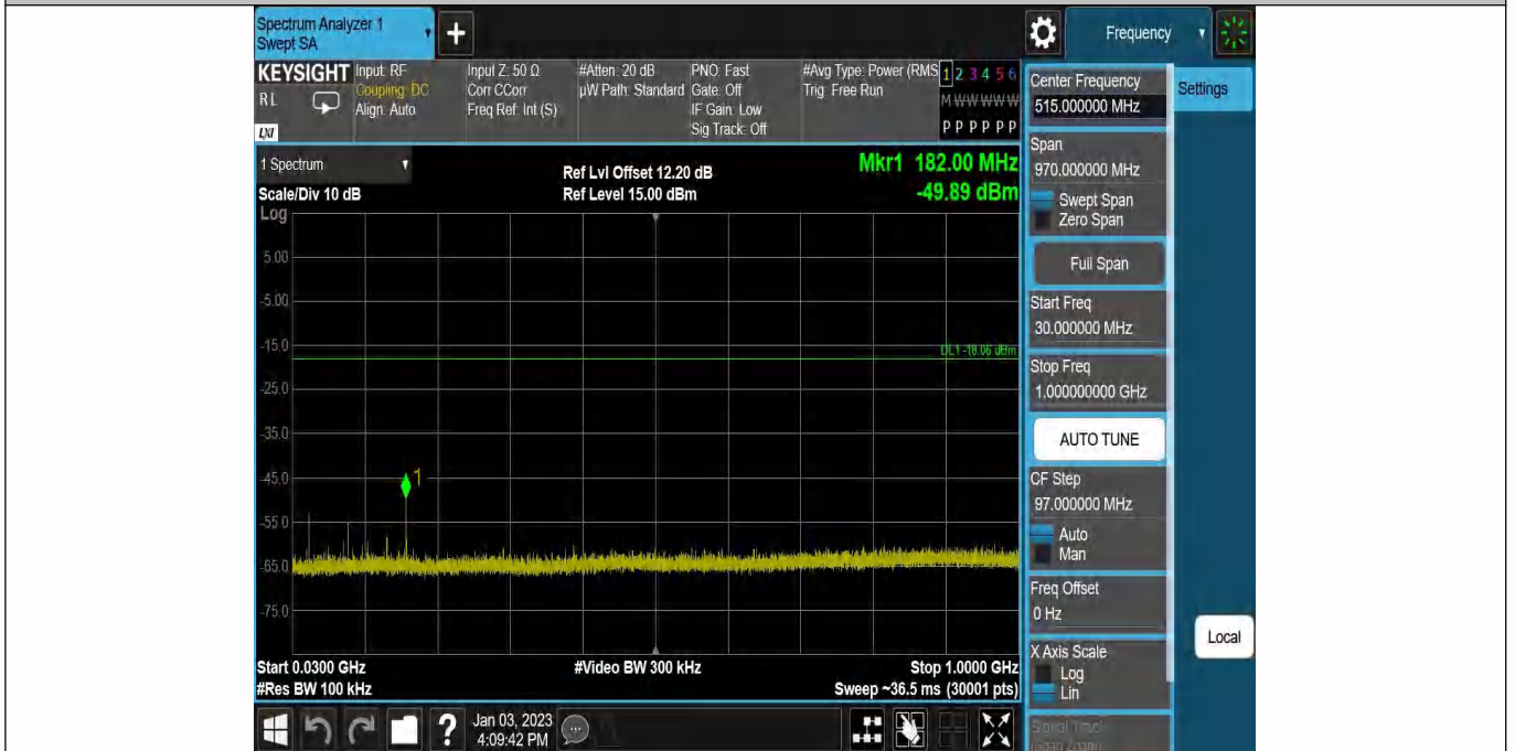
DH5-Ant1-2402-30~1000-1.94
