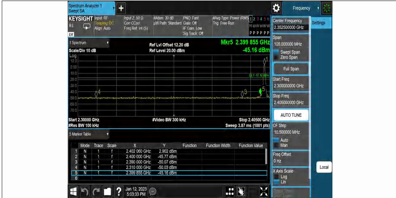
DH5-Ant1-Low-2402-2.90
