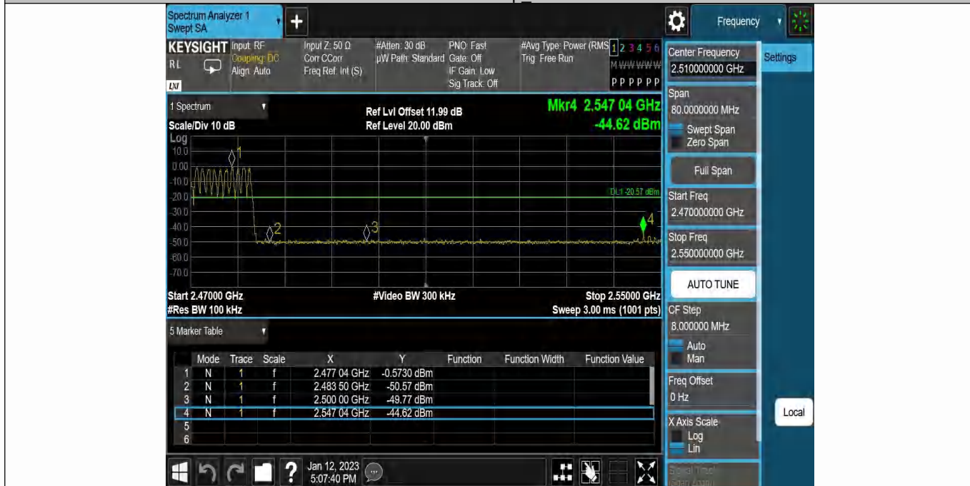
DH5-Ant1-High-Hop_2480--0.57
