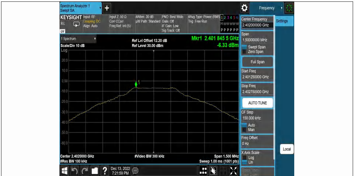
DH5-Ant1-2402-0~Reference--6.34
