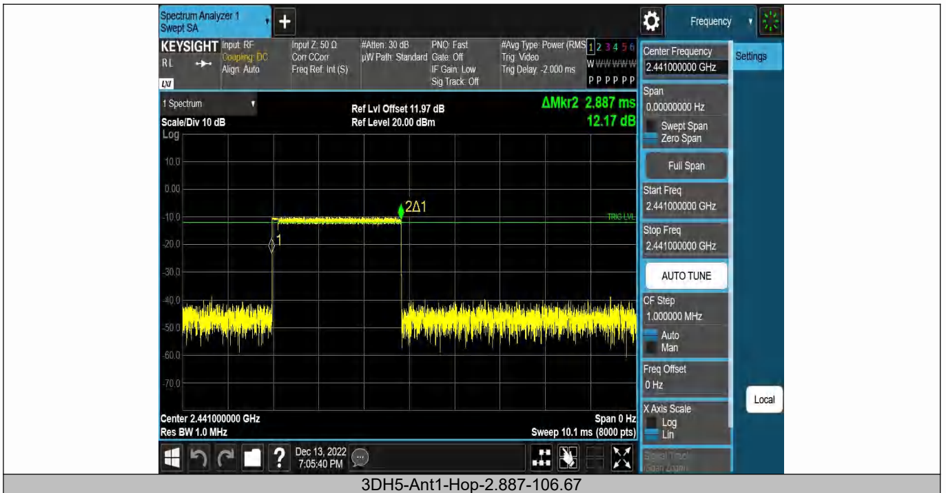
3DH5-Ant1-Hop-2.887-106.67
