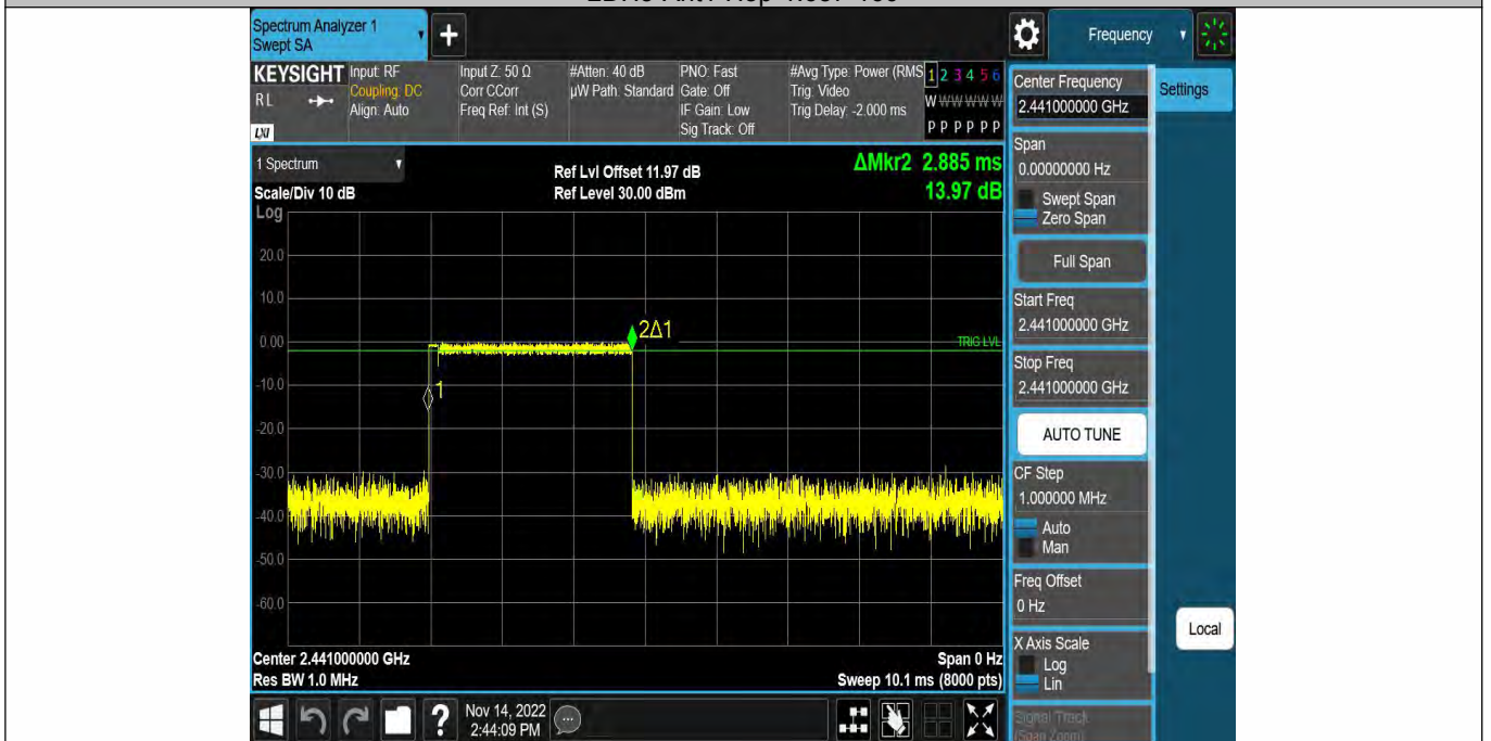
2DH5-Ant1-Hop-2.885-106.67
