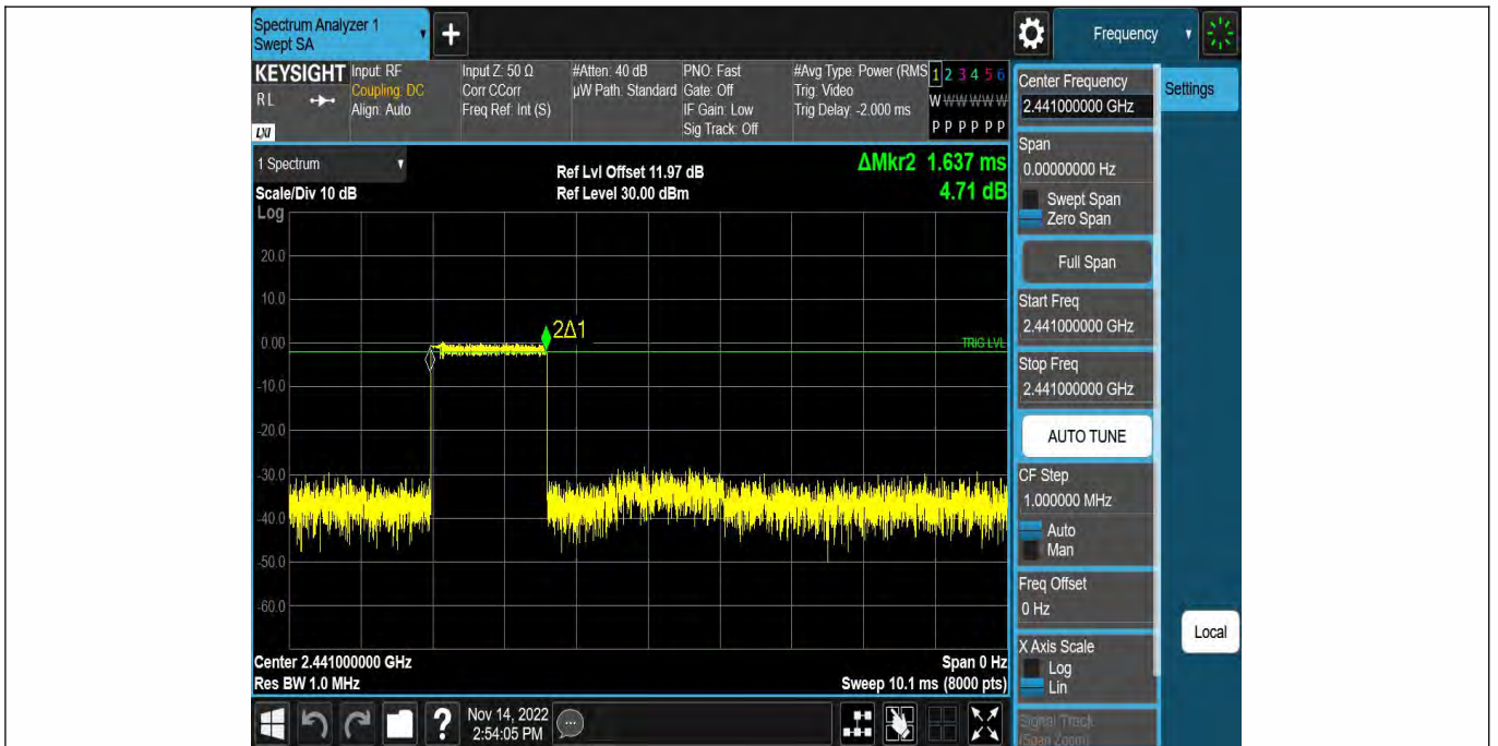
2DH3-Ant1-Hop-1.637-160
