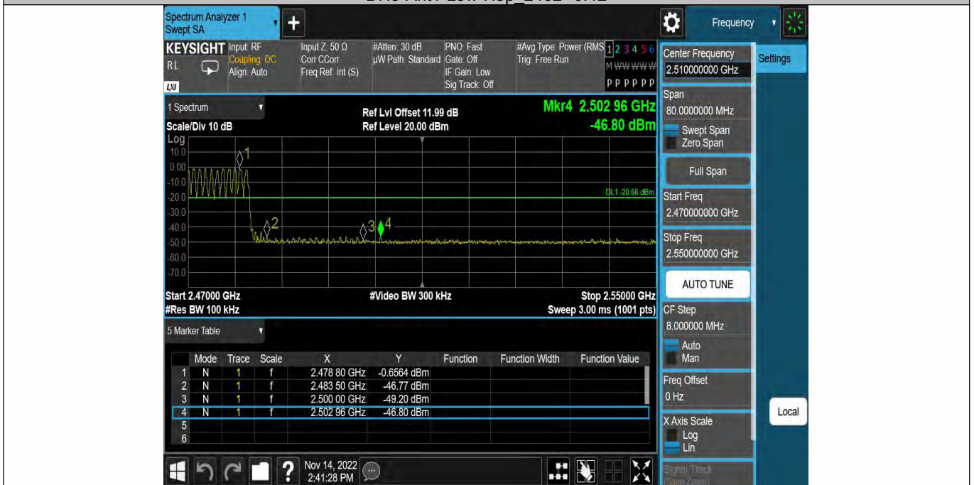
DH5-Ant1-High-Hop_2480--0.66
