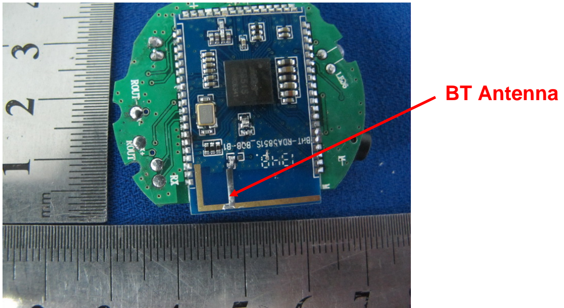
Photo 11 Internal of EUT
