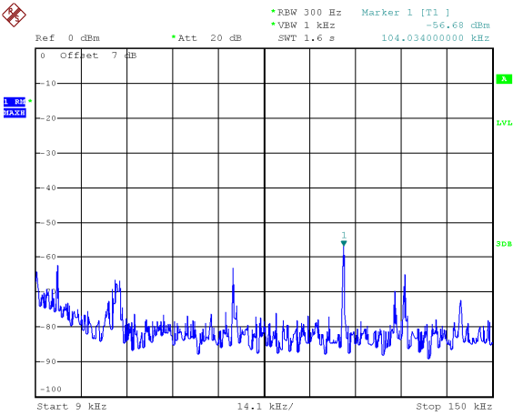
Mode: TX 11b channel 2
