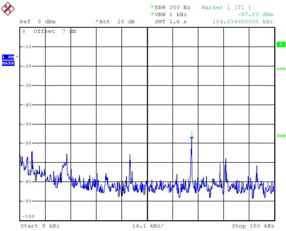
Mode: TX 11b channel 4
