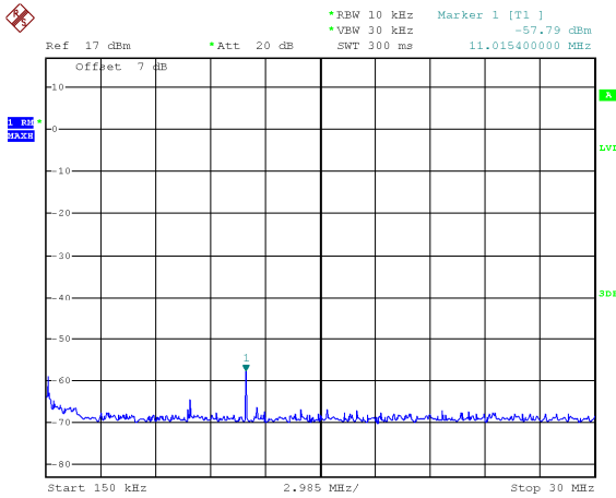
Mode: TX 11 n HT20 channel 2
