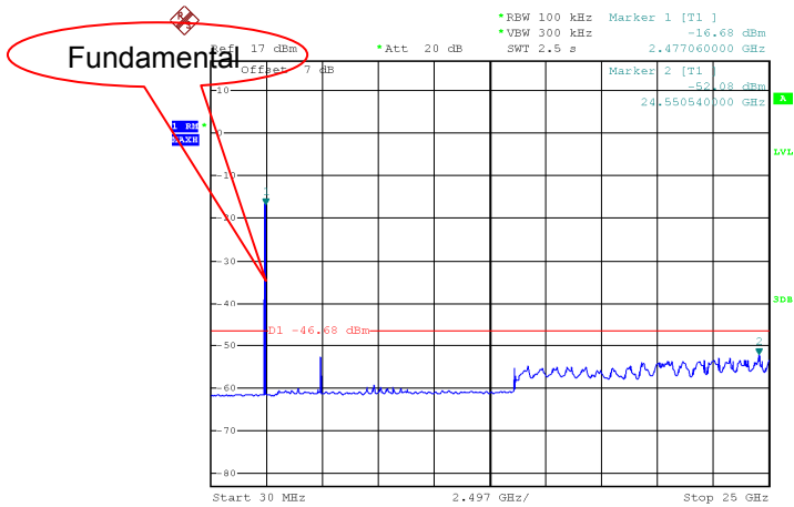
Mode: TX 11 n HT20 channel 4
