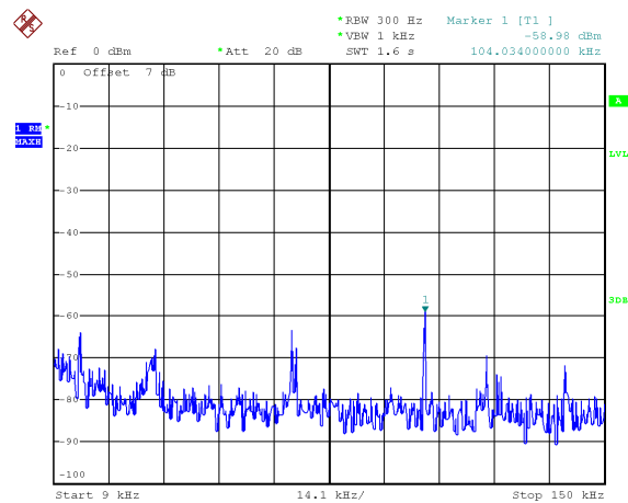
Mode: TX 11g channel 2
