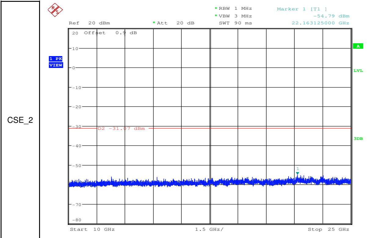
RF Conducted Spurious Emissions_11N40SISO_2452_Ant2
