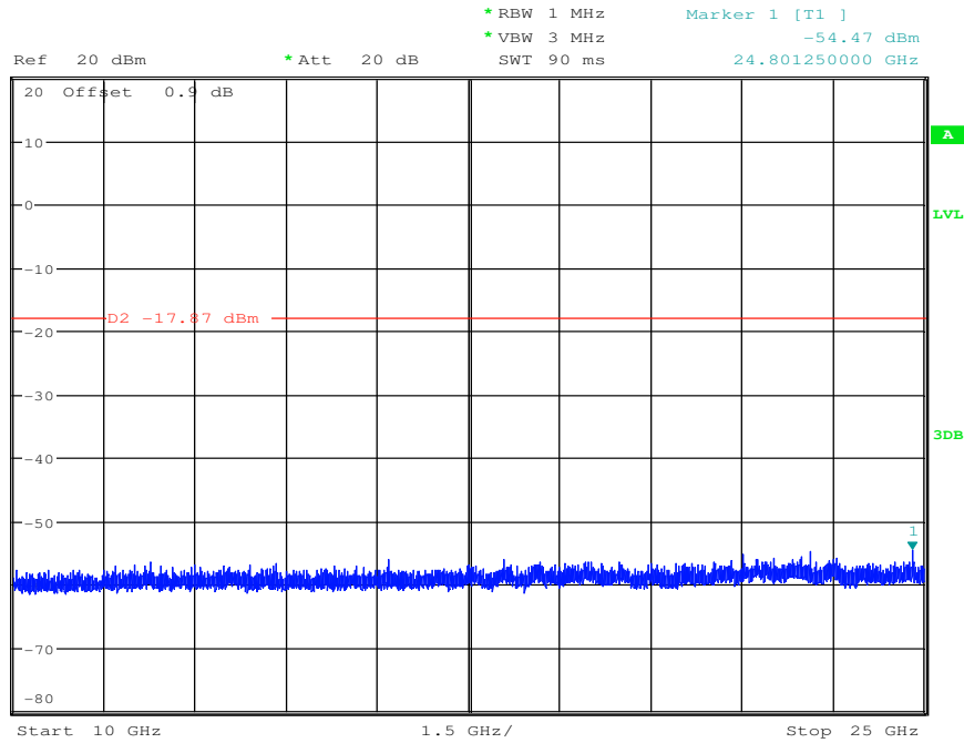
RF Conducted Spurious Emissions_11B_2462_Ant2
