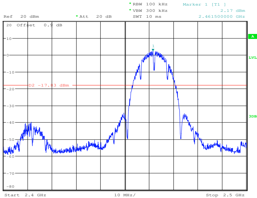
RF Conducted Spurious Emissions_11B_2462_Ant2
