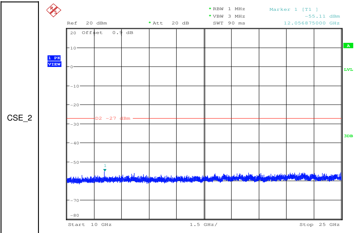
RF Conducted Spurious Emissions_11G_2412_Ant2
