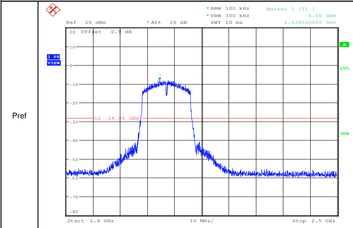
RF Conducted Spurious Emissions_11N20SISO_2437_Ant2
