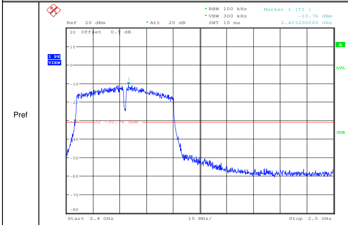
RF Conducted Spurious Emissions_11N40SISO_2422_Ant2
