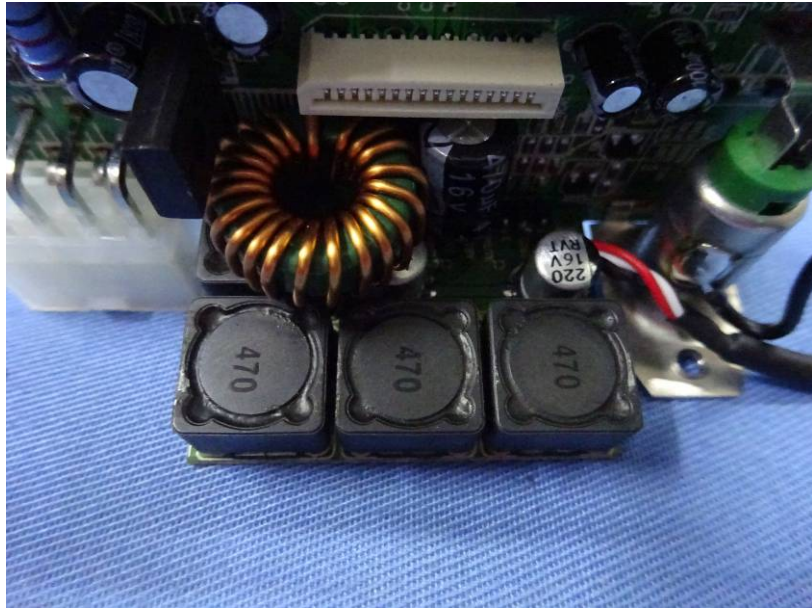
AMPLIFIER BOARD
