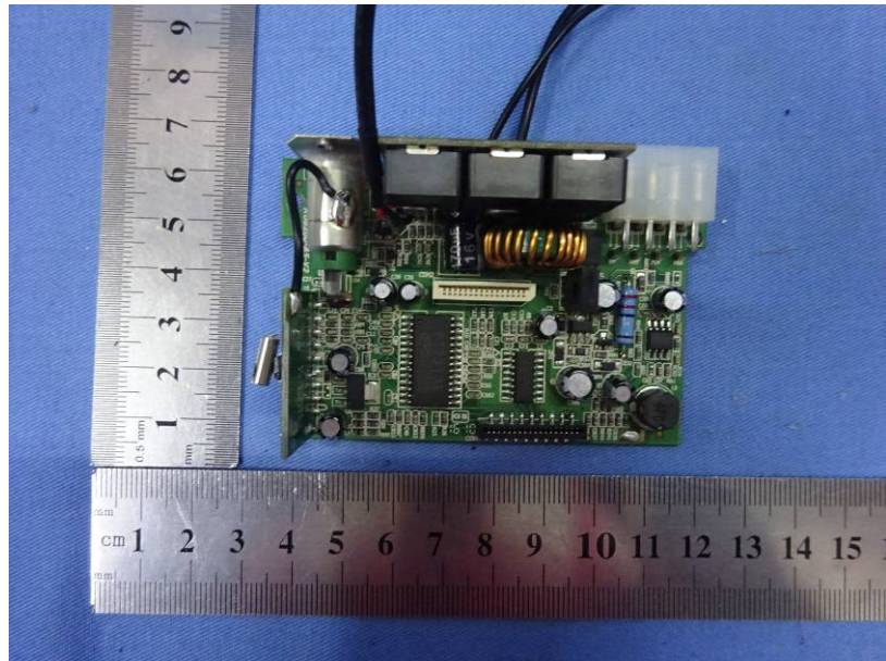
MAIN BOARD
