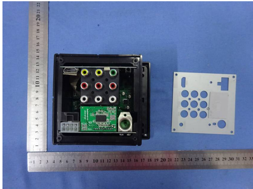
Uncover View
