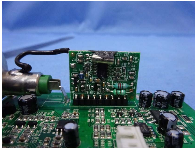
RECEIVE BOARD
