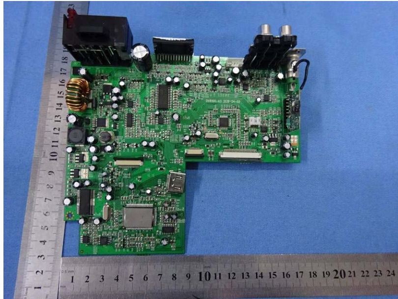
MAIN
