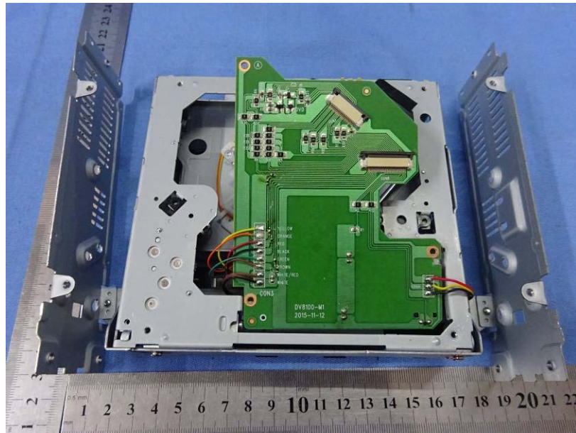
DVD mechanism
