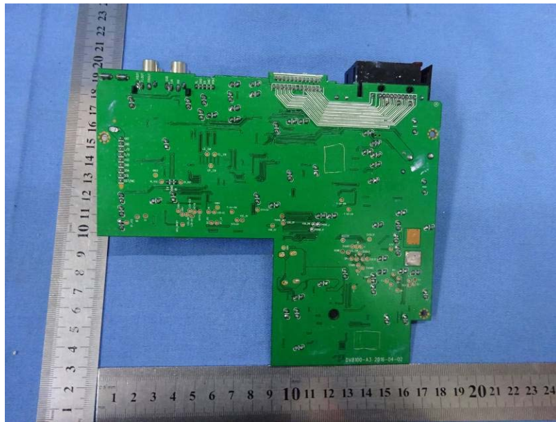
MAIN BOARD
