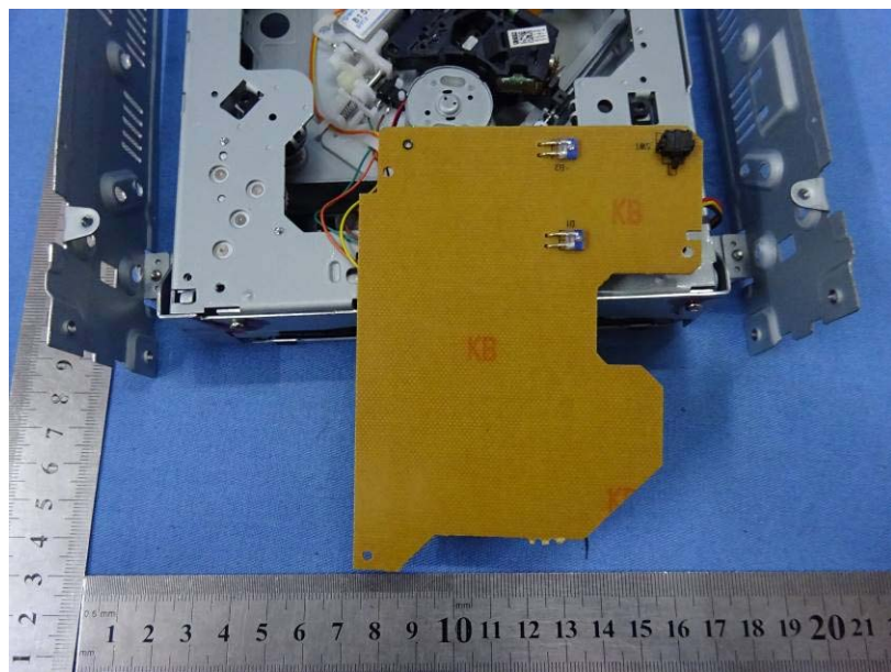
Connect Board
