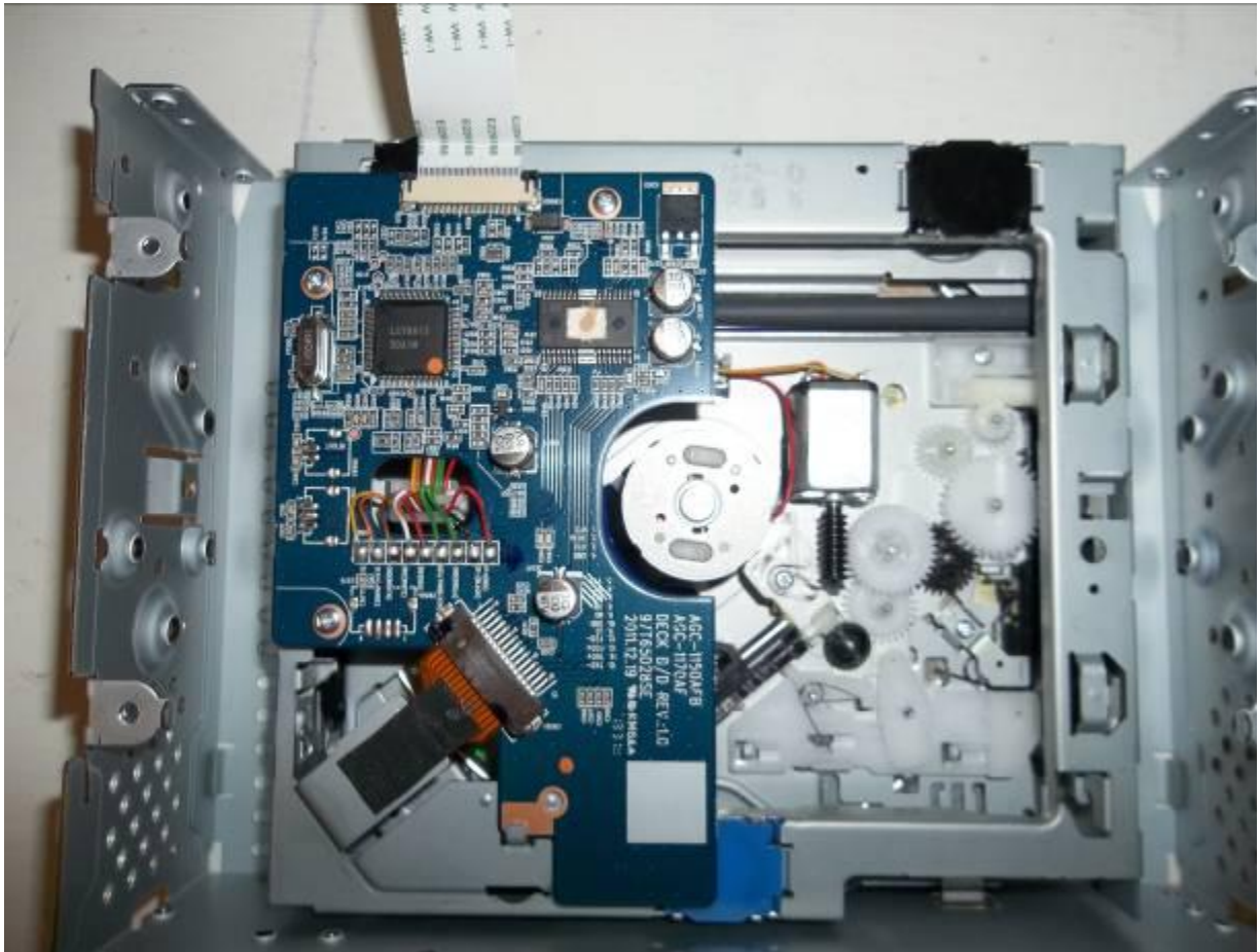
Figure 6. CD Player Control Board, Top
