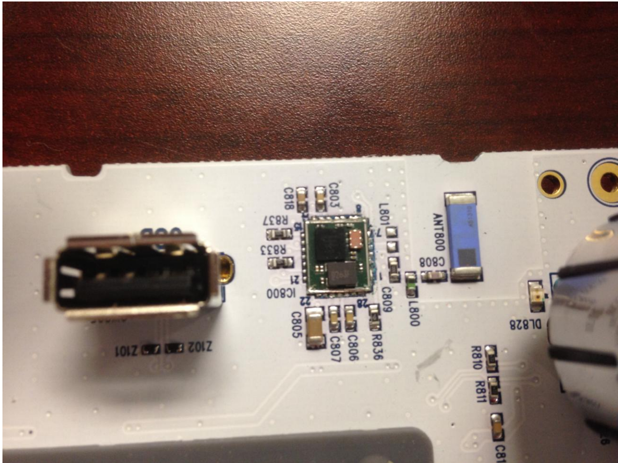
Figure 3. RF Radio Circuit (Close Up, RF shield removed)
