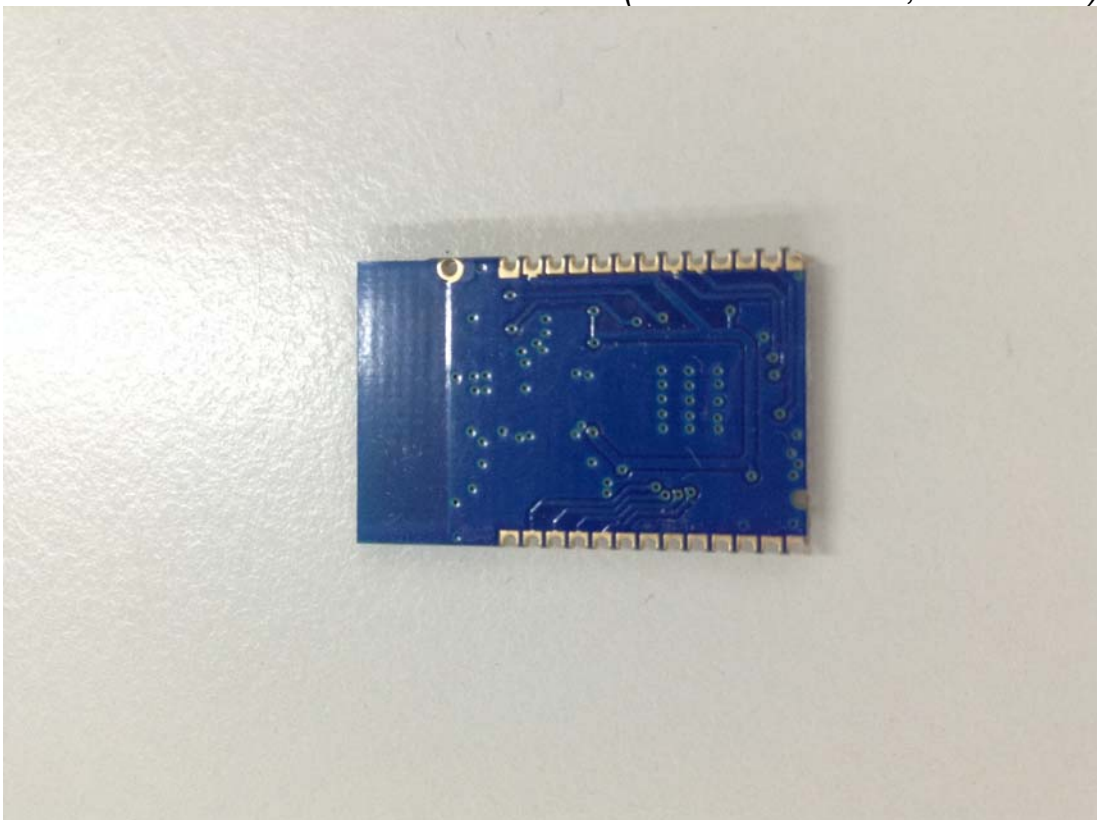
Figure 14 Internal View (RF Module Board, Back View)
