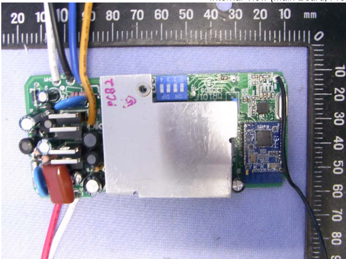
Photo 4 Internal View (Main Board, Front View)
