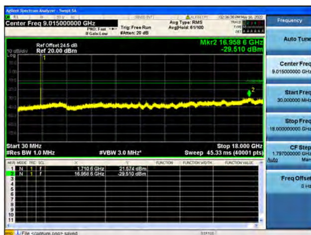
Band66 / 10MHz / Low CH / 64QAM
