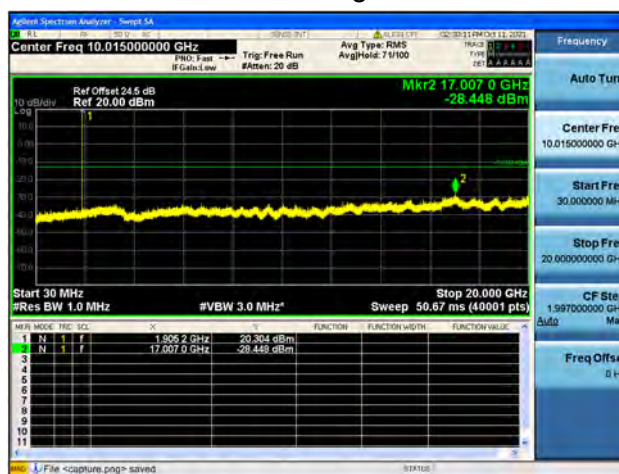
Band25 / 10MHz / High CH / 64QAM
