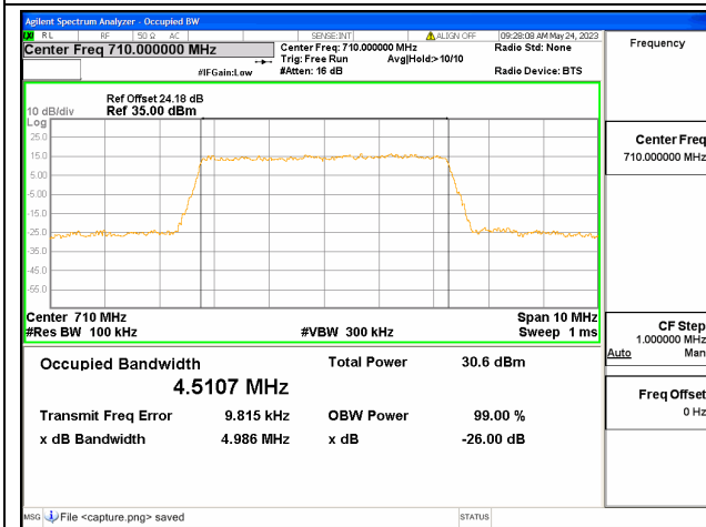
Band17 / 5MHz / 16QAM/ Mid CH
