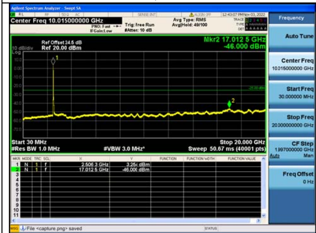
Band41C-30M-20G / 15MHz+20MHz / 75RB+100RB/ QPSK / LOW CH
