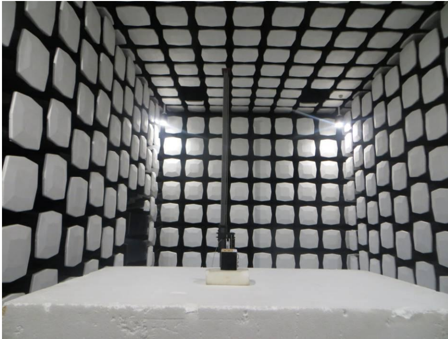
7. Radiated Emissions (Part 15C) (18-26.5GHz)
