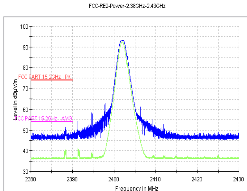
Fig.18. Radiated Emission Power (GFSK, Ch0, 2380MHz~2430MHz)
