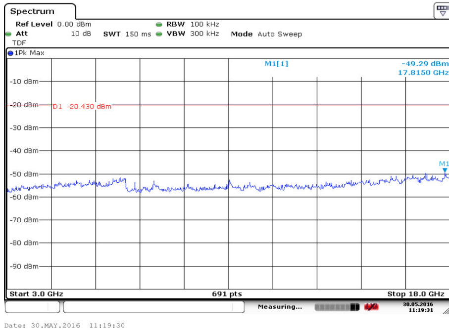
Fig.8. Conducted Spurious Emission (Ch19, 3 GHz-18 GHz)
