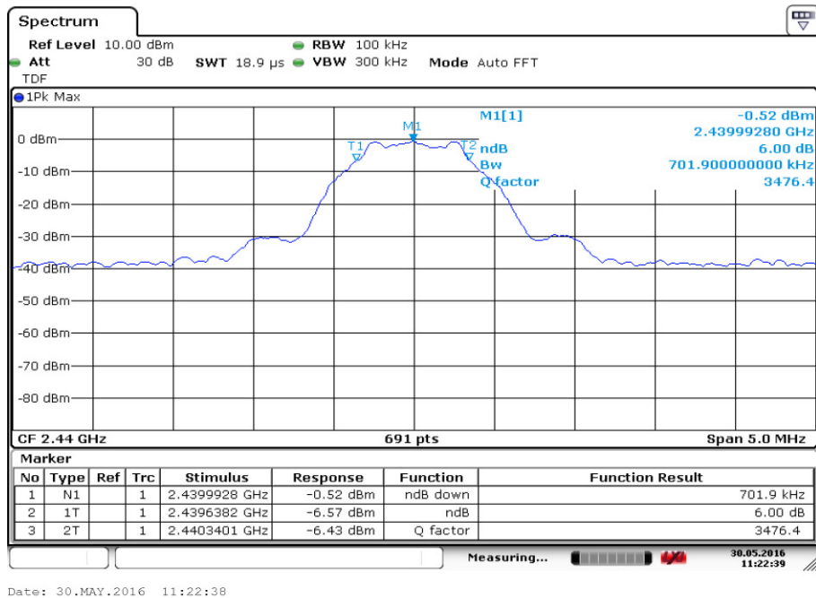
Fig.22. 6dB Bandwidth: GFSK, 2440 MHz
