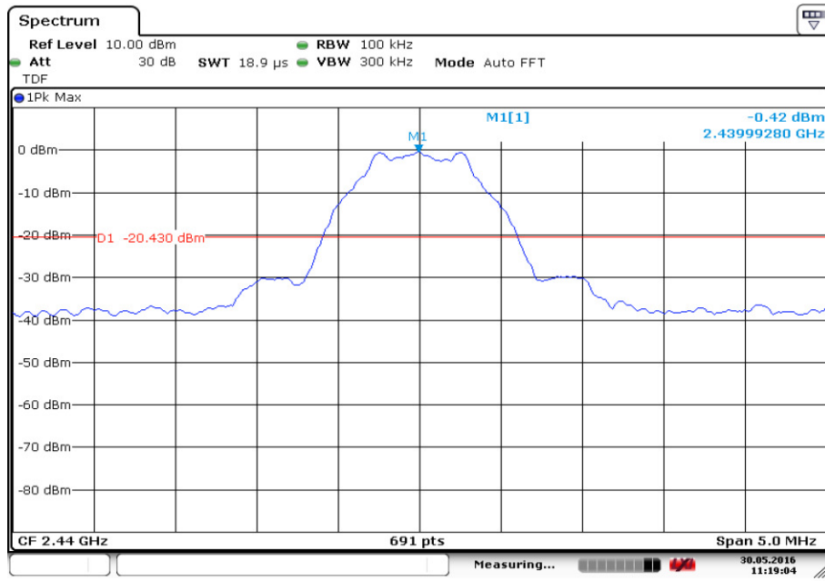
Fig.6. Conducted Spurious Emission (Ch19, Center Frequency)
