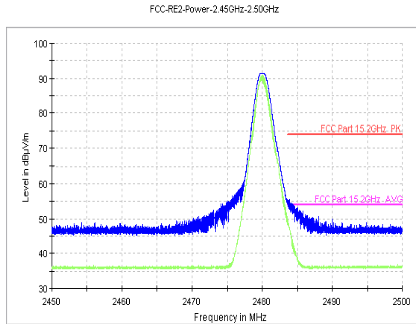
Fig.19. Radiated Emission Power (GFSK, Ch39, 2450MHz~2500MHz)
