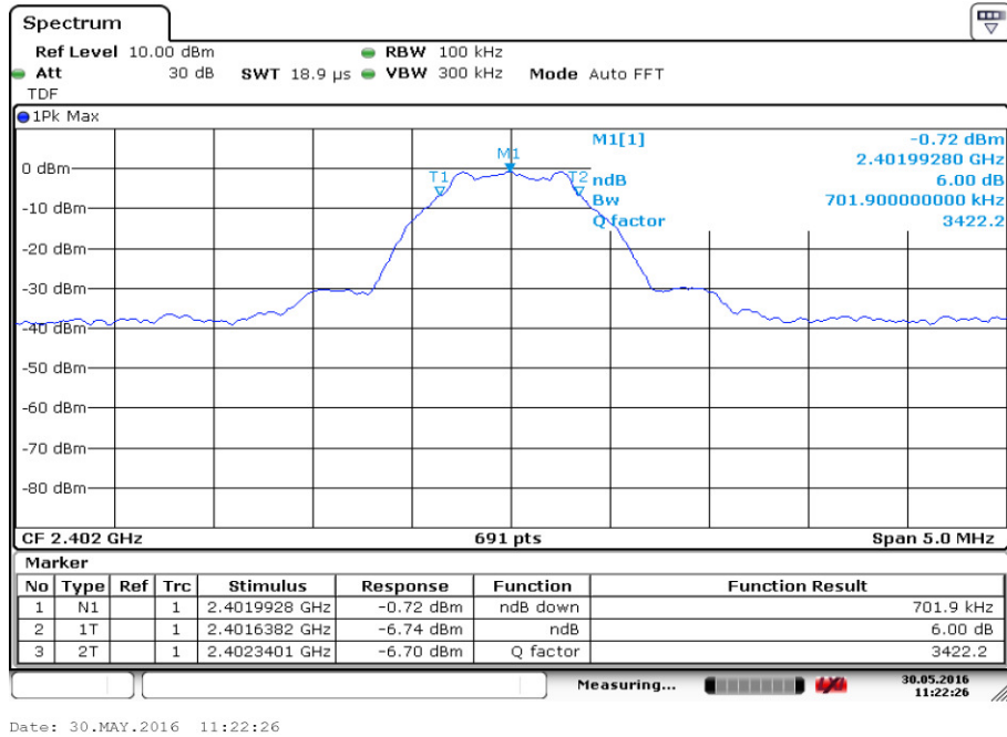
Fig.21. 6dB Bandwidth: GFSK, 2402 MHz
