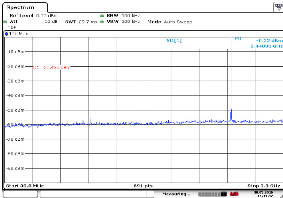
Fig.7. Conducted Spurious Emission (Ch19, 30 MHz-3 GHz)
