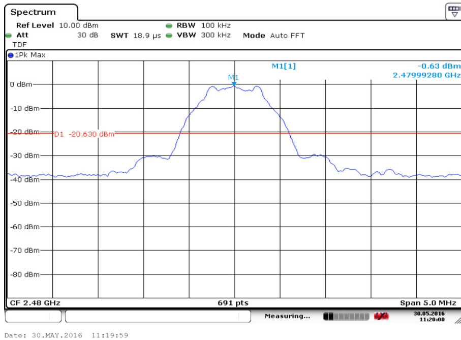
Fig.9. Conducted Spurious Emission (Ch39, Center Frequency)
