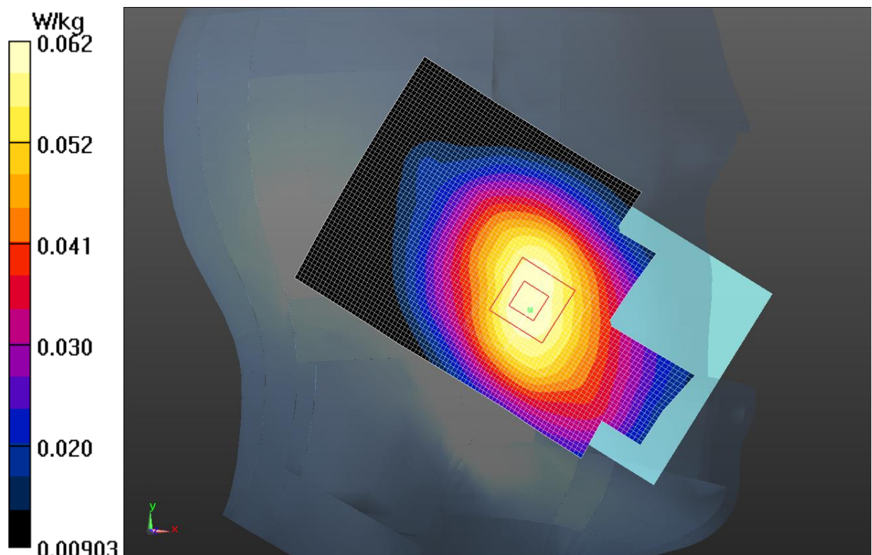
Fig.19 LTE Band 17
