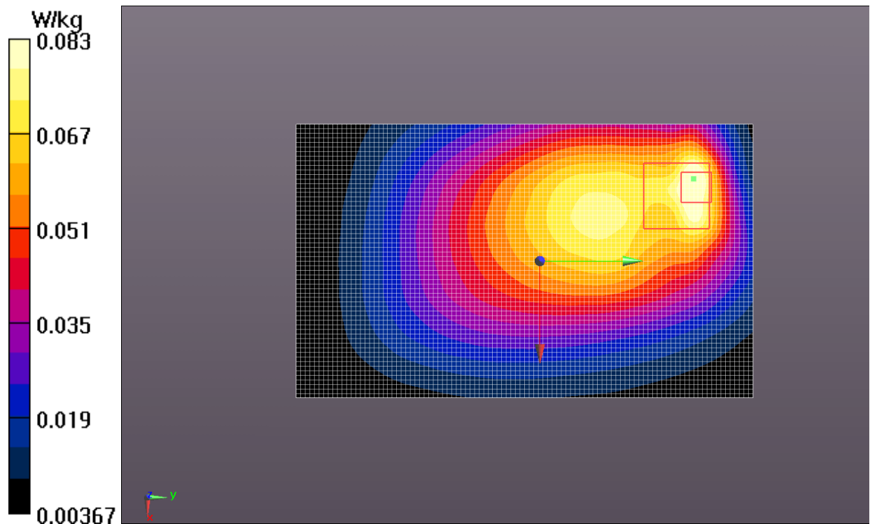
Fig.18 LTE Band 12
