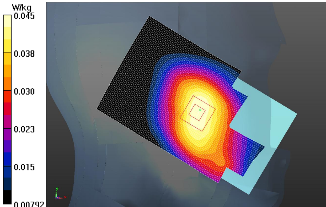
Fig.17 LTE Band 12
