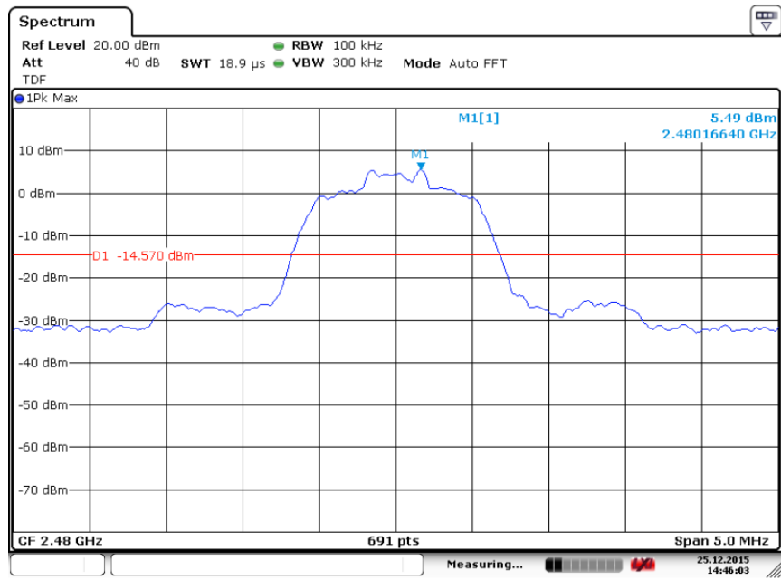
Fig. 37 Conducted Spurious Emission ( \pi/4 DQPSK, Ch78, 2.480GHz)
