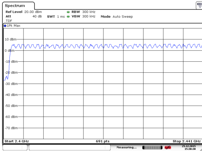
Fig. 91 Hopping channel ch0~39 (8DPSK, Ch39)
