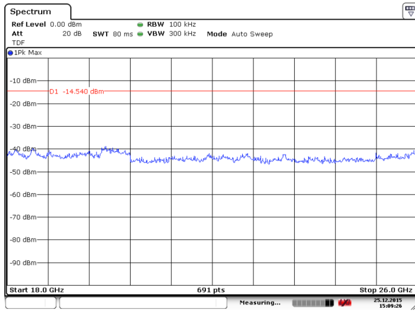
Fig. 49 Conducted Spurious Emission (All channel, 18 GHz-26 GHz)
