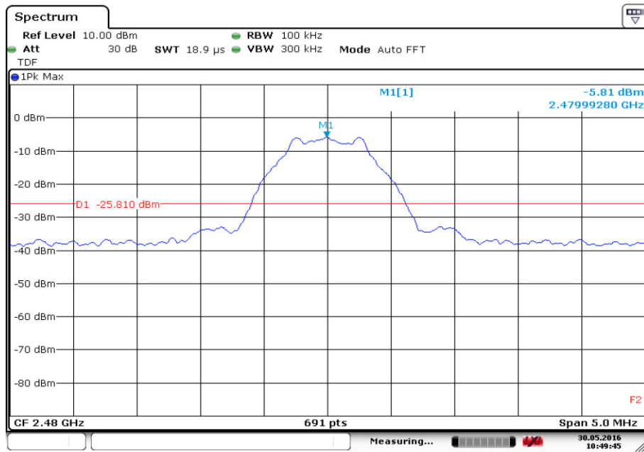
Fig.9. Conducted Spurious Emission (Ch39, Center Frequency)
