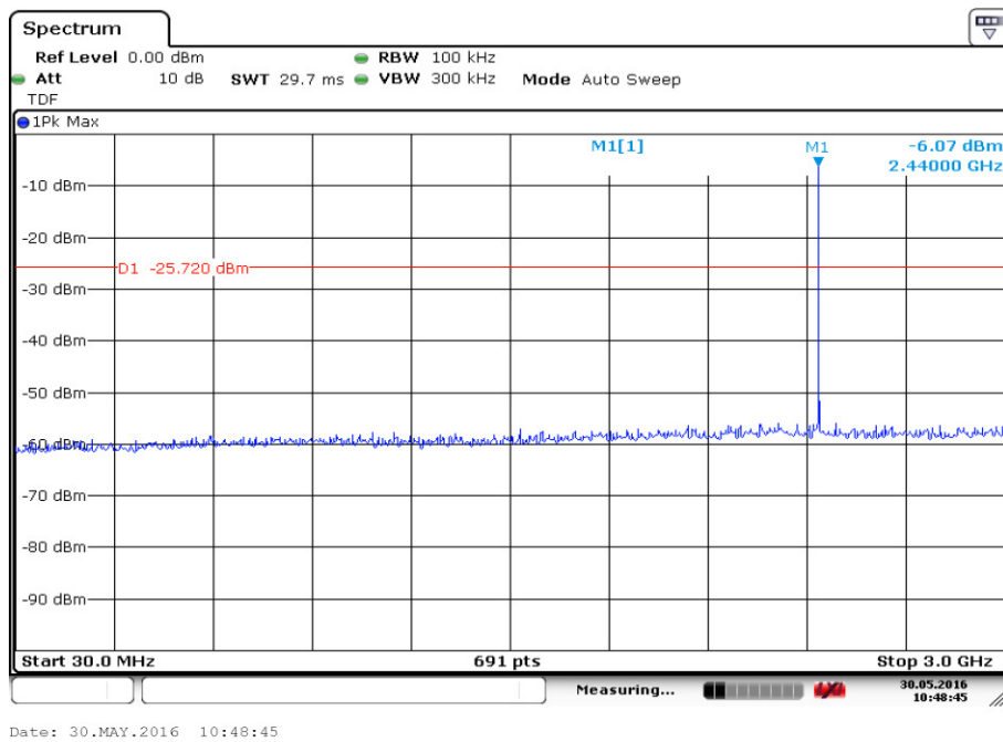
Fig.7. Conducted Spurious Emission (Ch19, 30 MHz-3 GHz)
