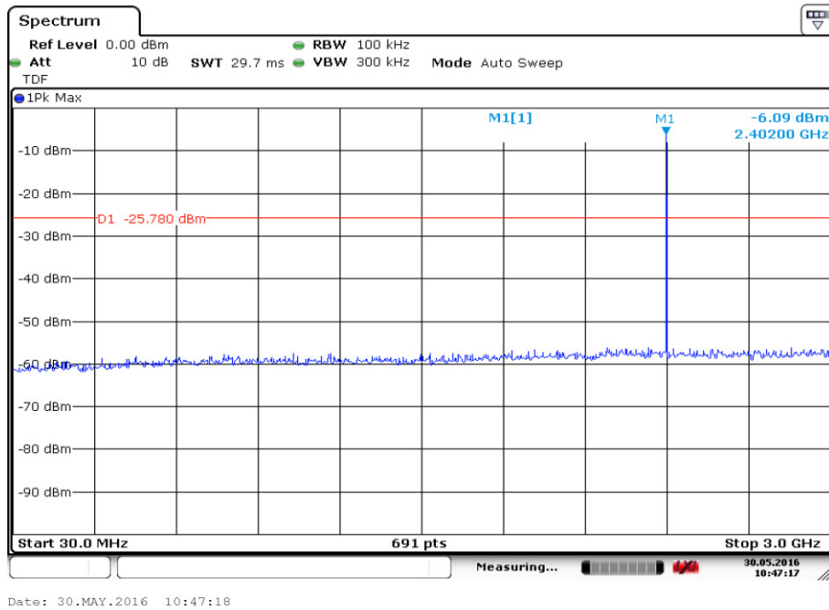
Fig.4. Conducted Spurious Emission (Ch0, 30 MHz-3 GHz)
