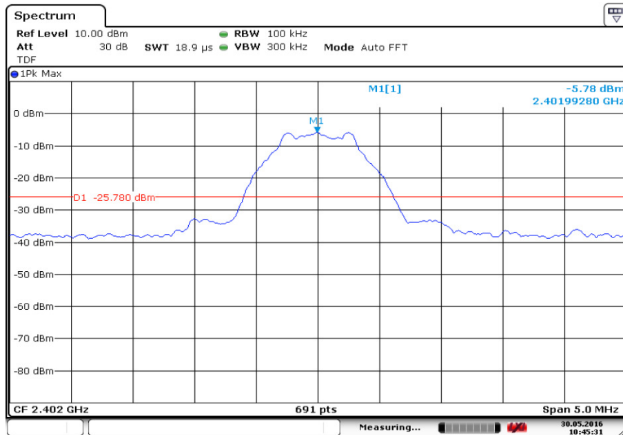
Fig.3. Conducted Spurious Emission (Ch0, Center Frequency)
