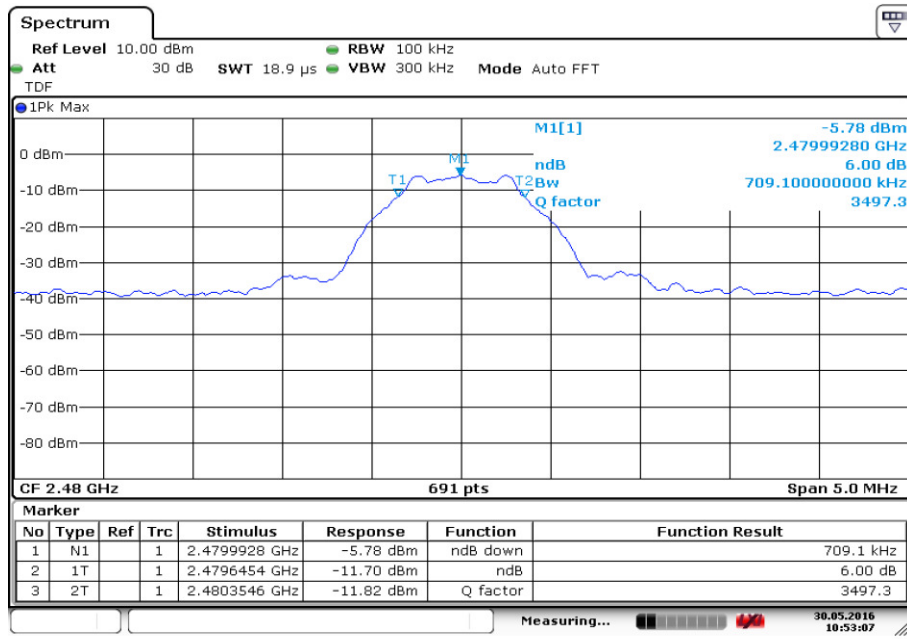
Fig.23. 6dB Bandwidth: GFSK, 2480 MHz
