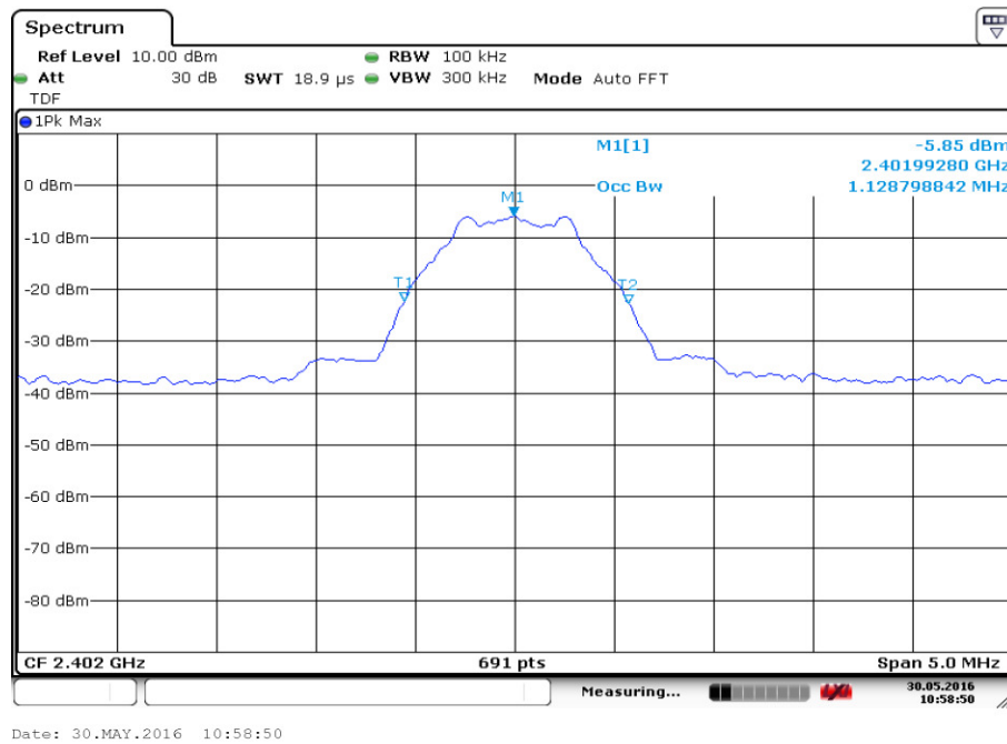
Fig.27. Occupied Bandwidth: GFSK, 2402 MHz
