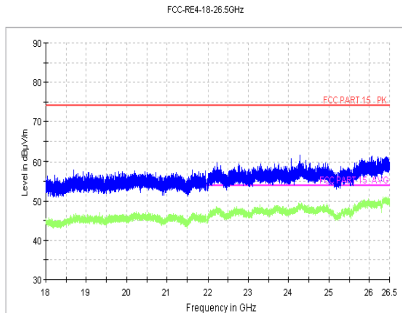
Fig.20. Radiated emission: 18 GHz – 26.5 GHz
