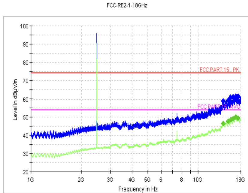
Fig.17. Radiated Spurious Emission (Ch39, 1 GHz-18 GHz)
