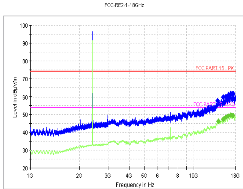
Fig.13. Radiated Spurious Emission (GFSK, Ch0, 1 GHz ~18 GHz)
