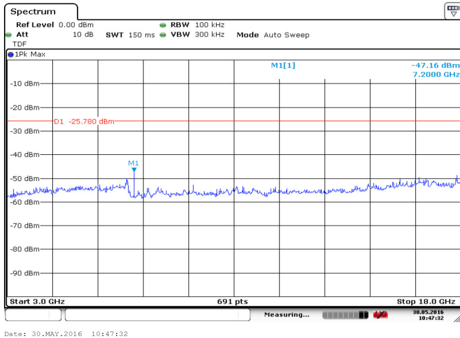
Fig.5. Conducted Spurious Emission (Ch0, 3 GHz-18 GHz)
