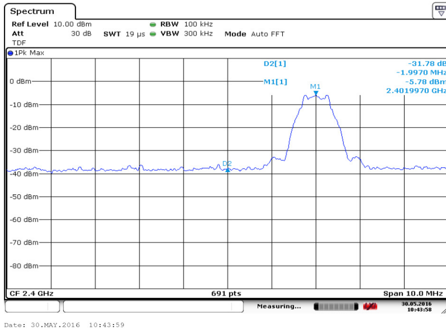
Fig.1. Frequency Band Edges: GFSK, 2402 MHz, Hopping Off
