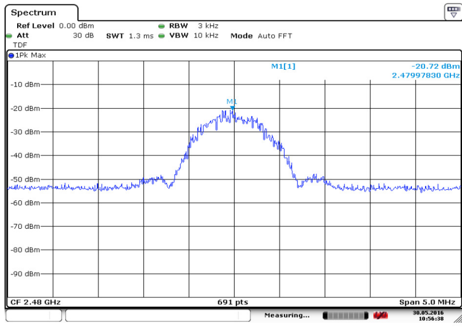
Fig.26. Maximum Power Spectral Density Level Function: GFSK, 2480 MHz
