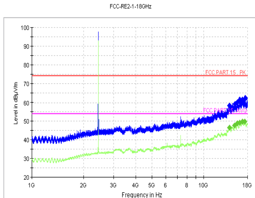
Fig.16. Radiated Spurious Emission (Ch19, 1 GHz-18 GHz)
