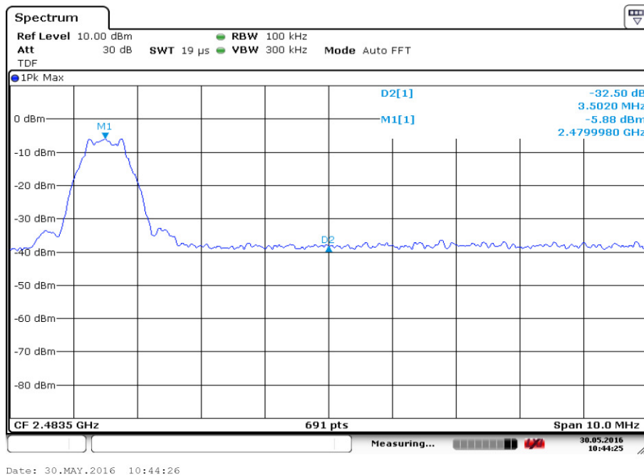
Fig.2. Frequency Band Edges: GFSK, 2480 MHz, Hopping Off
