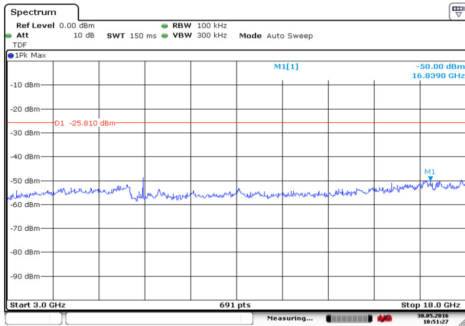
Fig.11. Conducted Spurious Emission (Ch39, 3 GHz-18 GHz)
