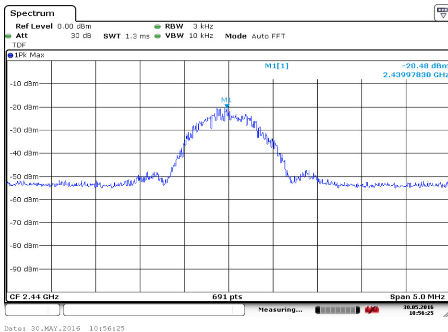
Fig.25. Maximum Power Spectral Density Level Function: GFSK, 2440 MHz
