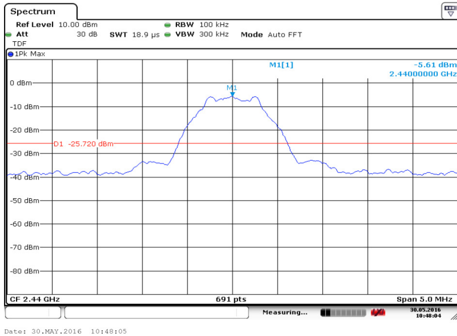
Fig.6. Conducted Spurious Emission (Ch19, Center Frequency)
