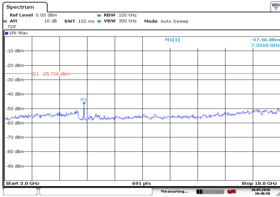
Fig.8. Conducted Spurious Emission (Ch19, 3 GHz-18 GHz)
