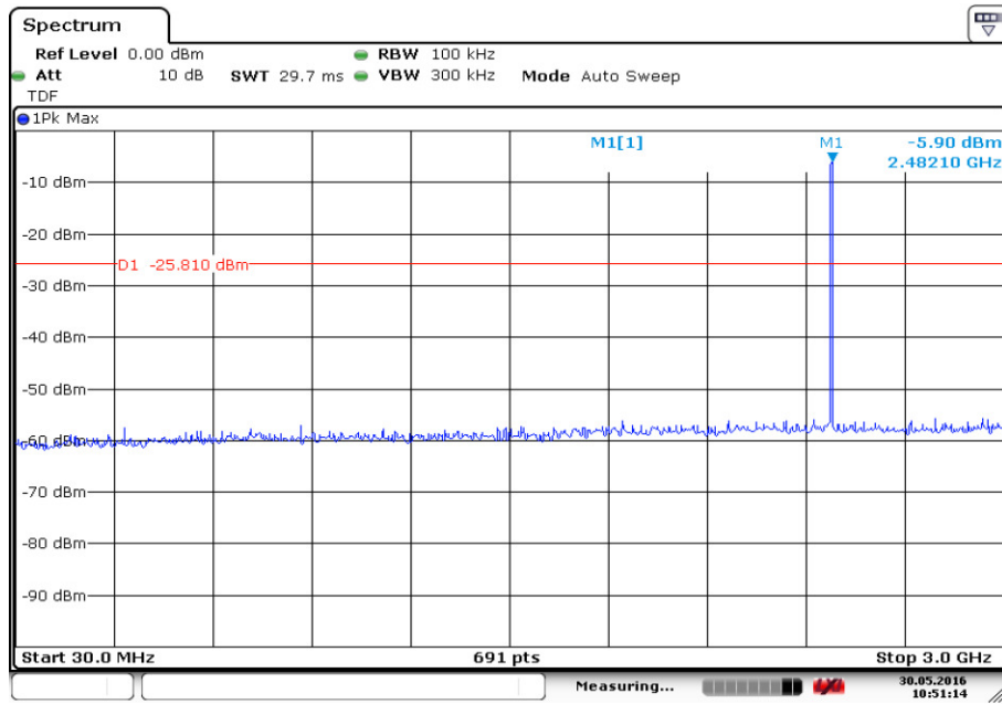
Fig.10. Conducted Spurious Emission (Ch39, 30 MHz-3 GHz)
