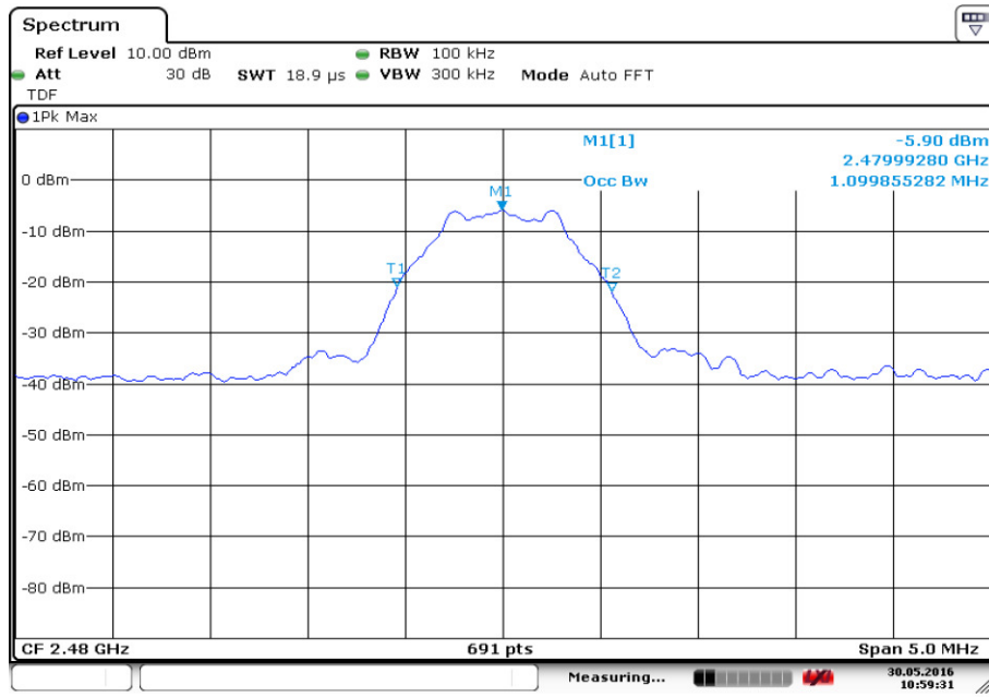
Fig.29. Occupied Bandwidth: GFSK, 2480 MHz
