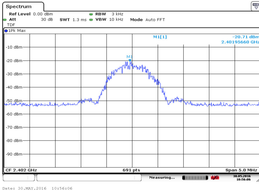
Fig.24. Maximum Power Spectral Density Level Function: GFSK, 2402 MHz
