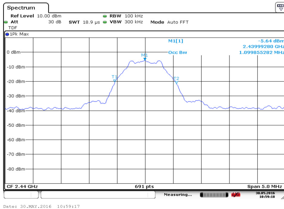
Fig.28. Occupied Bandwidth: GFSK, 2440 MHz
