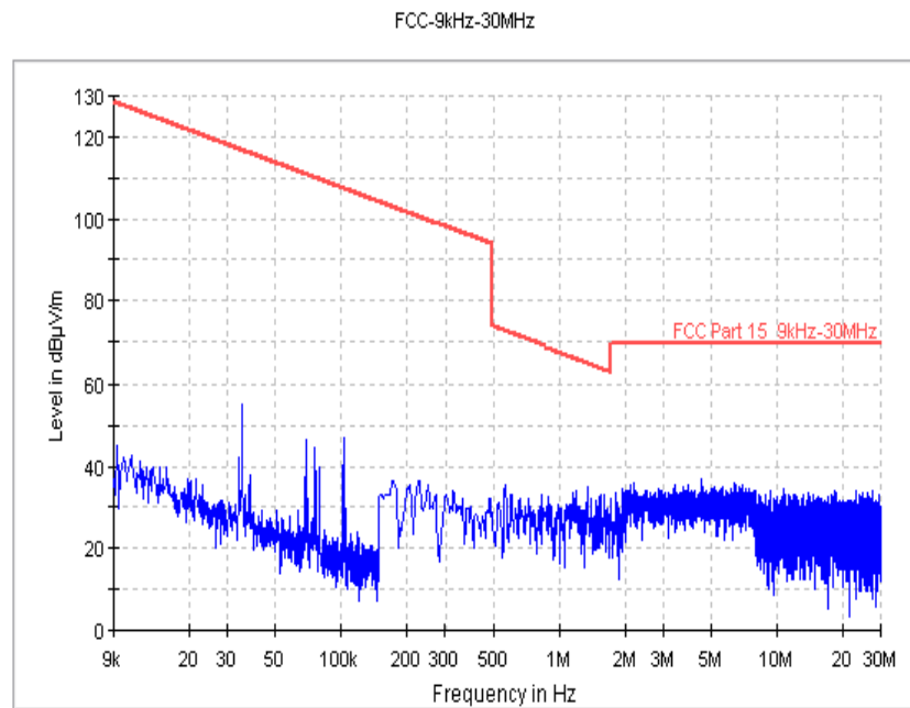
Fig.14. Radiated Spurious Emission (Ch19, 9 kHz-30 MHz)
