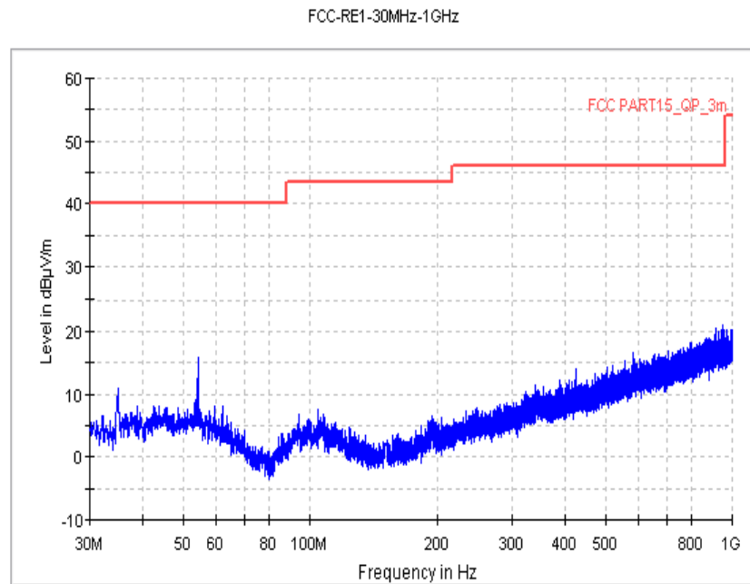
Fig.15. Radiated Spurious Emission (Ch19, 30 MHz-1 GHz)
