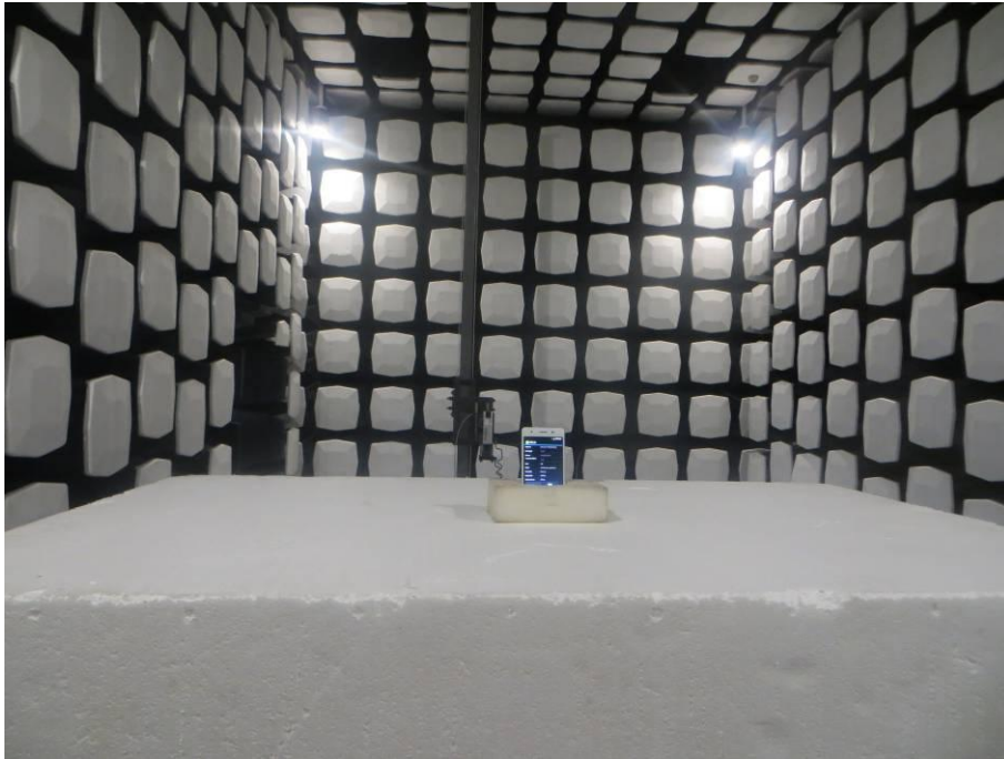
7. Radiated Emissions (Part 15C) (18GHz-26.5GHz)
