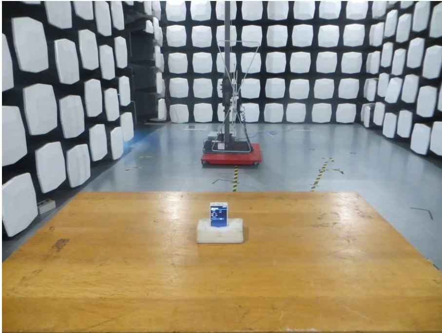
5. Radiated Emissions (Part 15C) (30MHz-1GHz)
