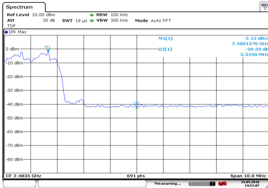
Fig.12. Frequency Band Edges: 8DPSK, Channel 78, Hopping On
