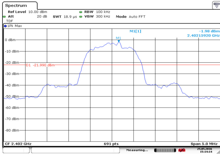
Fig.31. Conducted Spurious Emission (8DPSK, Ch0, 2.402GHz)
