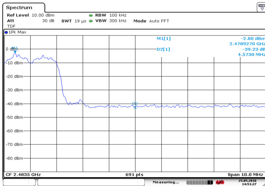
Fig.8. Frequency Band Edges: \pi/4 DQPSK, Channel 78, Hopping On
