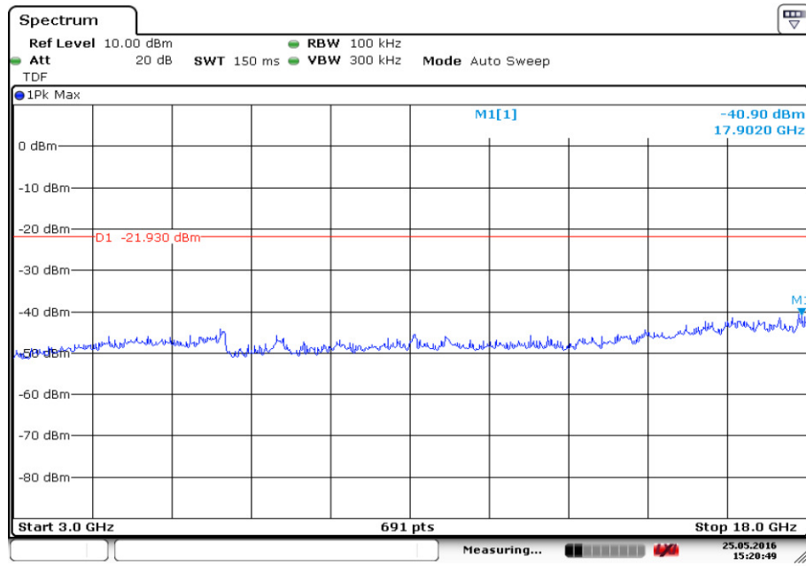
Fig.39. Conducted Spurious Emission (8DPSK, Ch78, 3GHz-18 GHz)
