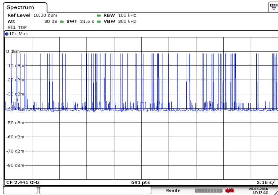
Fig.64. Number of Transmissions Measurement: Channel 39, Packet DH5
