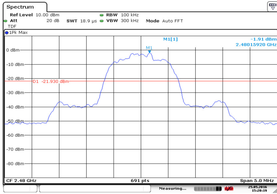
Fig.37. Conducted Spurious Emission (8DPSK, Ch78, 2.480GHz)
