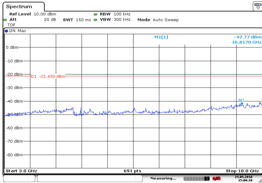
Fig.21. Conducted Spurious Emission (GFSK, Ch78, 3GHz-18 GHz)
