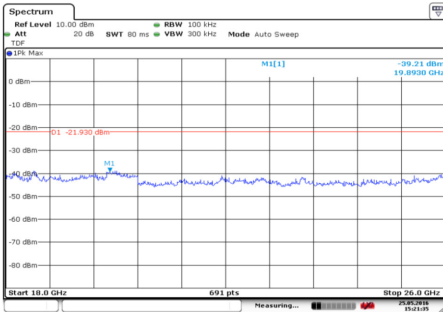
Fig.40. Conducted spurious emission: All Channel, 18GHz - 26GHz
