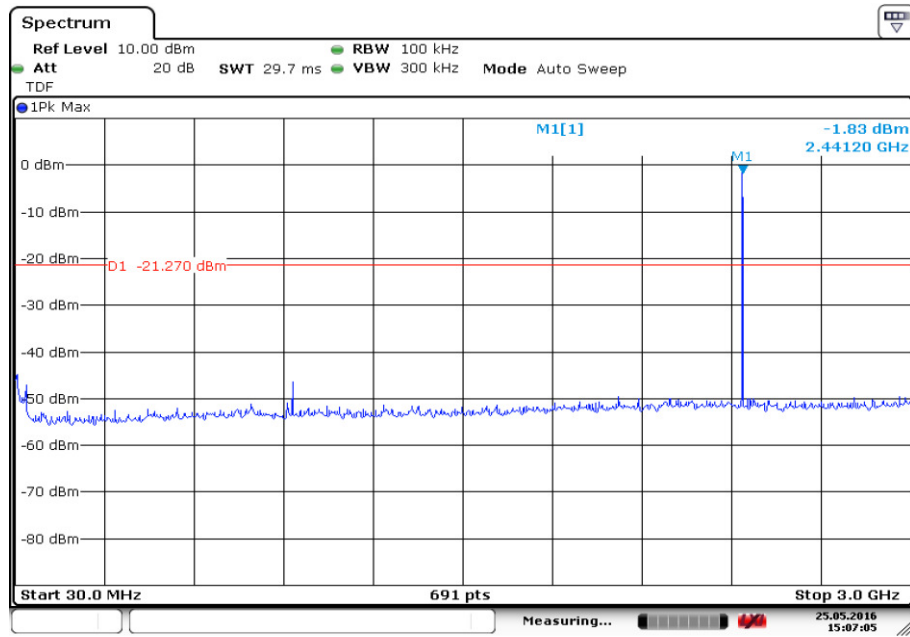
Fig.17. Conducted Spurious Emission (GFSK, Ch39, 30 MHz-3 GHz)
