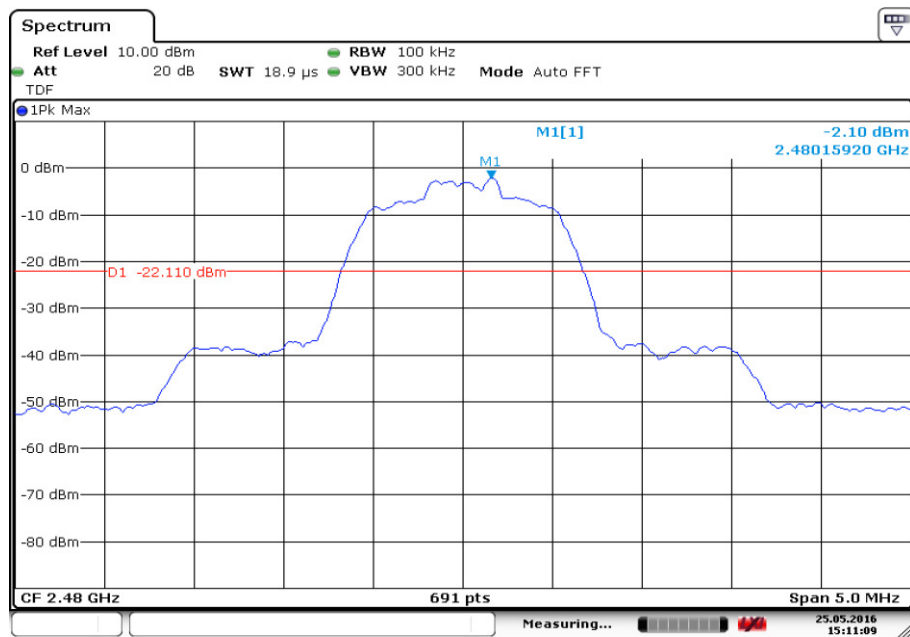
Fig.28. Conducted Spurious Emission ( \pi/4 DQPSK, Ch78, 2.480GHz)
