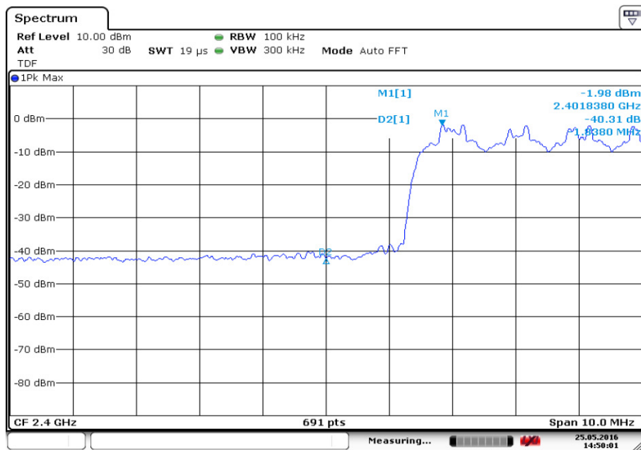
Fig.6. Frequency Band Edges: \pi/4 DQPSK, Channel 0, Hopping On
