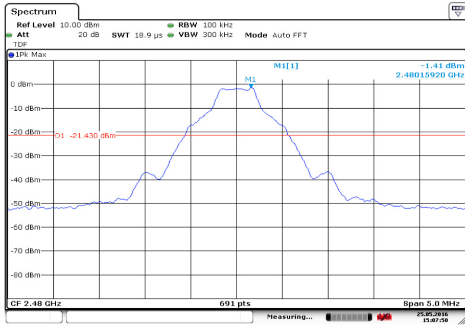
Fig.19. Conducted Spurious Emission (GFSK, Ch78, 2.480GHz)
