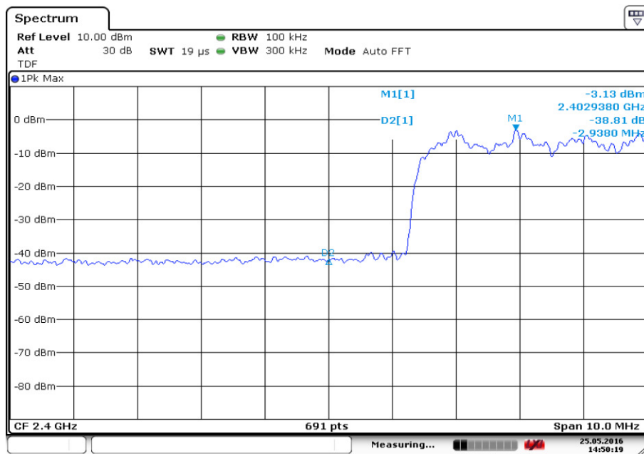
Fig.10. Frequency Band Edges: 8DPSK, Channel 0, Hopping On
