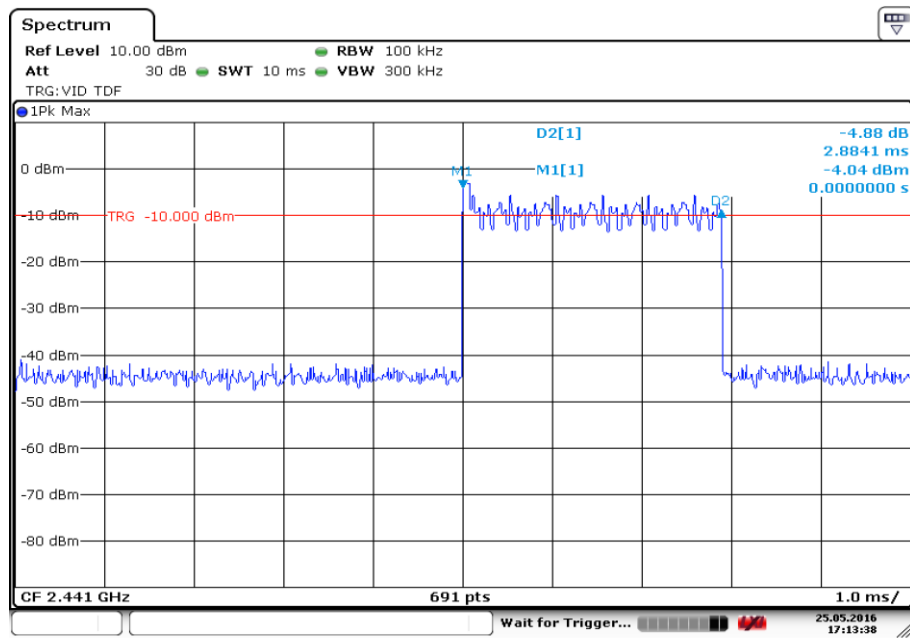
Fig.67. Time of occupancy (Dwell Time): Channel 39, Packet 3-DH5
