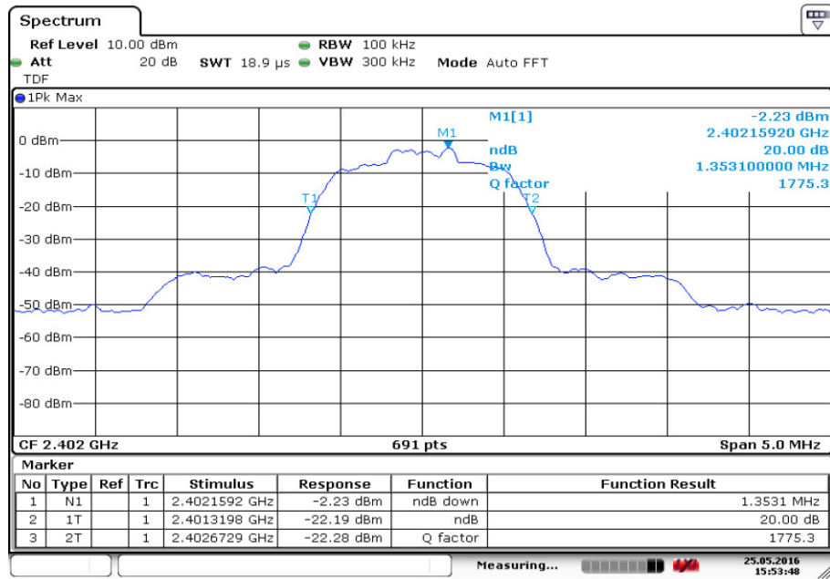
Fig.72. 20dB Bandwidth: \pi/4 DQPSK, Channel 0
