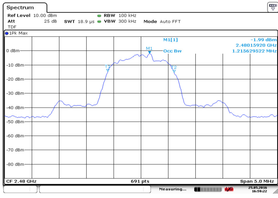
Fig.95. Occupied Bandwidth: 8DPSK, Channel 78
