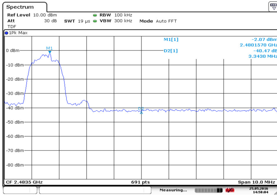
Fig.11. Frequency Band Edges: 8DPSK, Channel 78, Hopping Off
