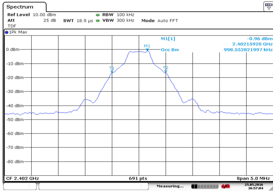
Fig.87. Occupied Bandwidth: GFSK, Channel 0
