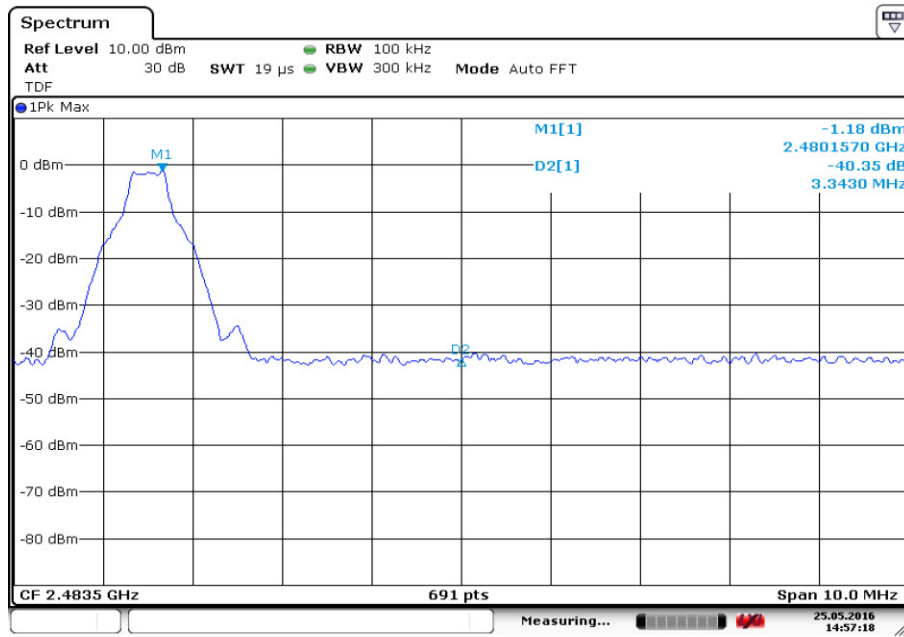
Fig.3. Frequency Band Edges: GFSK, Channel 78, Hopping Off
