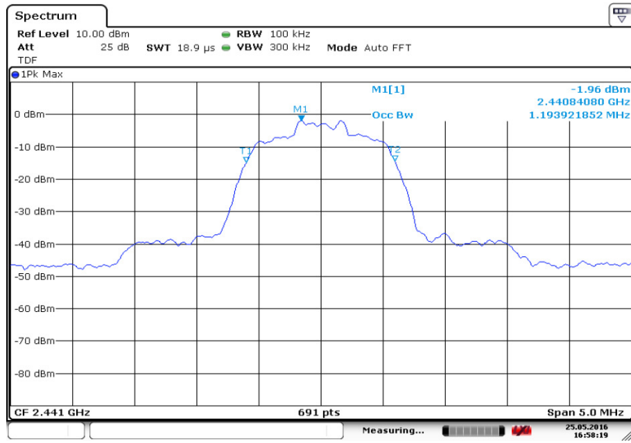
Fig.91. Occupied Bandwidth: \pi/4 DQPSK, Channel 39
