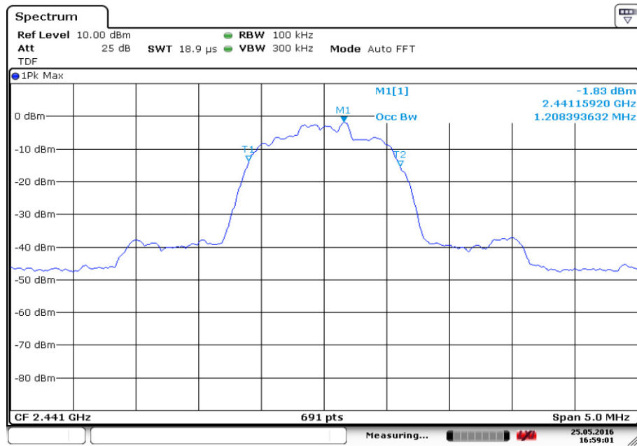
Fig.94. Occupied Bandwidth: 8DPSK, Channel 39
