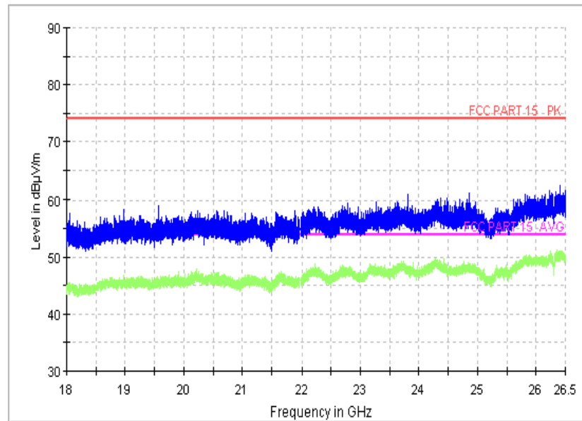
Fig.62. Radiated Spurious Emission (All channel, 18 GHz ~26.5 GHz)
