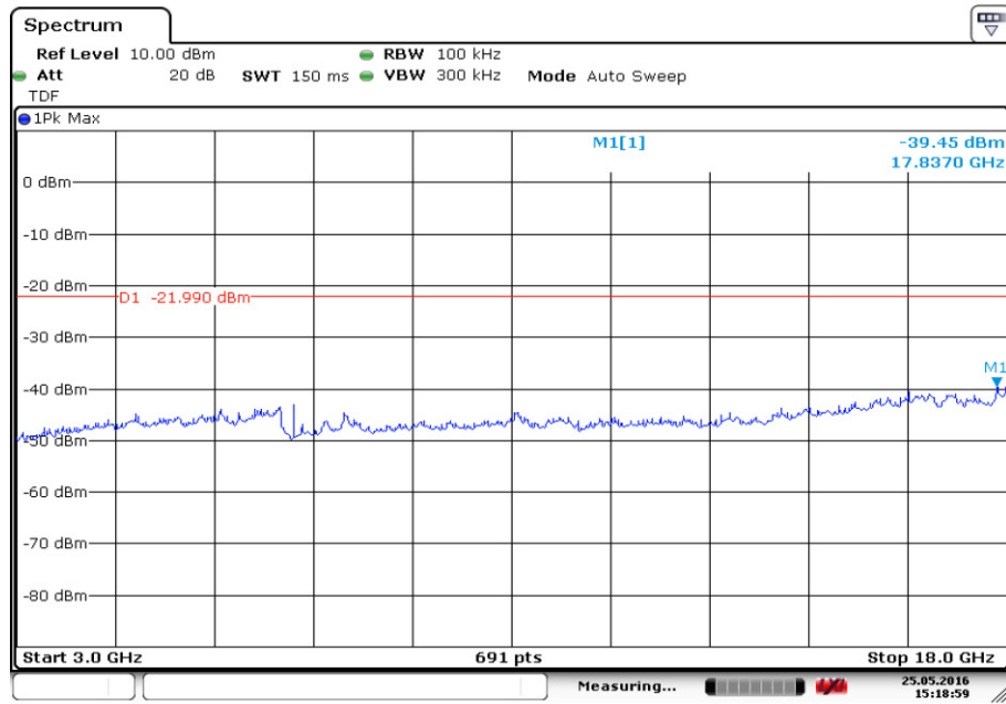
Fig.33. Conducted Spurious Emission (8DPSK, Ch0, 3GHz-18 GHz)
