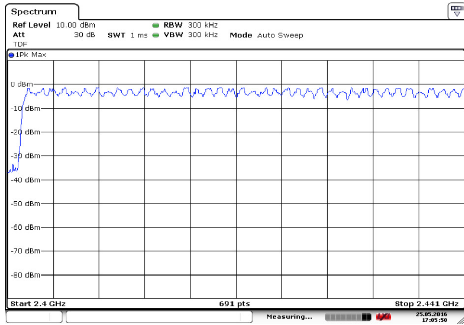
Fig.85. Number of hopping frequencies: 8DPSK, Channel 0 - 39
