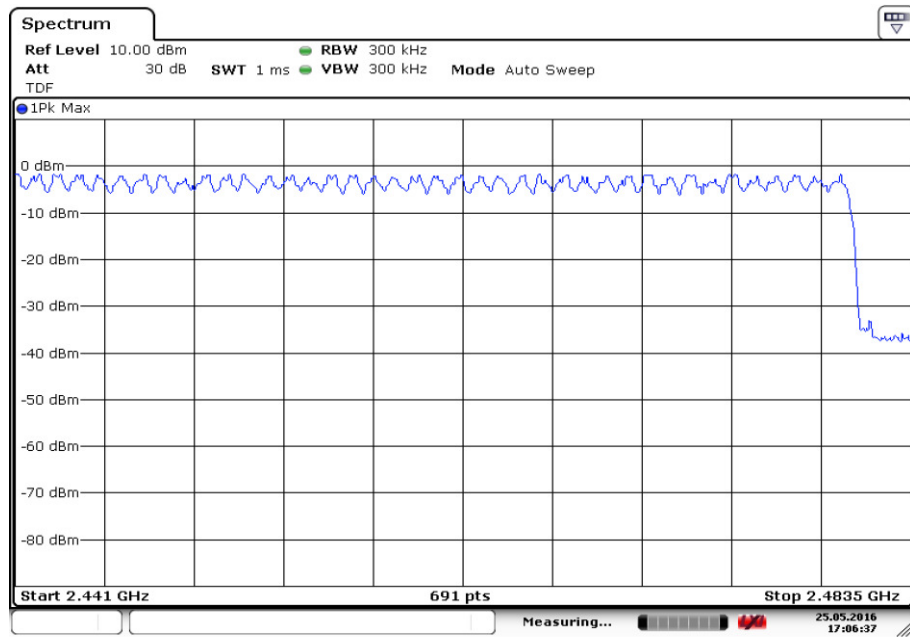
Fig.86. Number of hopping frequencies: 8DPSK, Channel 40 - 78
