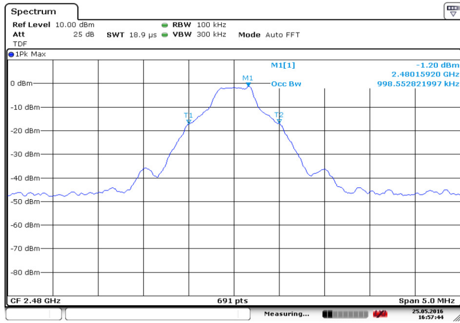
Fig.89. Occupied Bandwidth: GFSK, Channel 78
