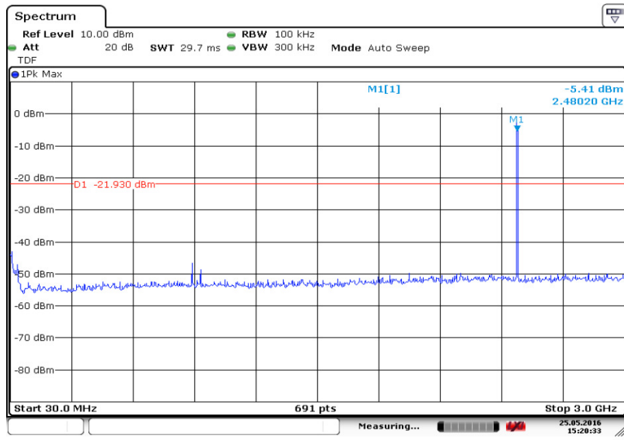
Fig.38. Conducted Spurious Emission (8DPSK, Ch78, 30 MHz-3 GHz)
