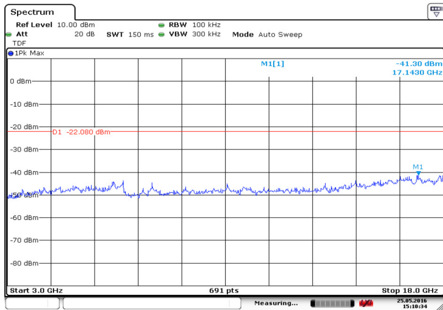
Fig.27. Conducted Spurious Emission ( \pi/4 DQPSK, Ch39, 3GHz-18 GHz)
