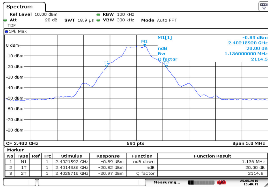
Fig.69. 20dB Bandwidth: GFSK, Channel 0
