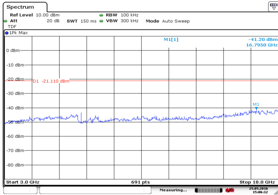
Fig.15. Conducted Spurious Emission (GFSK, Ch0, 3GHz-18 GHz)
