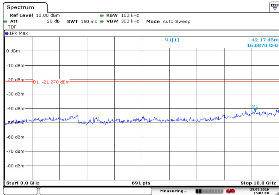
Fig.18. Conducted Spurious Emission (GFSK, Ch39, 3GHz-18 GHz)
