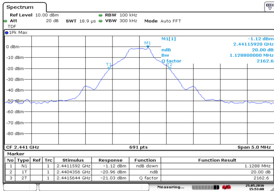
Fig.70. 20dB Bandwidth: GFSK, Channel 39
