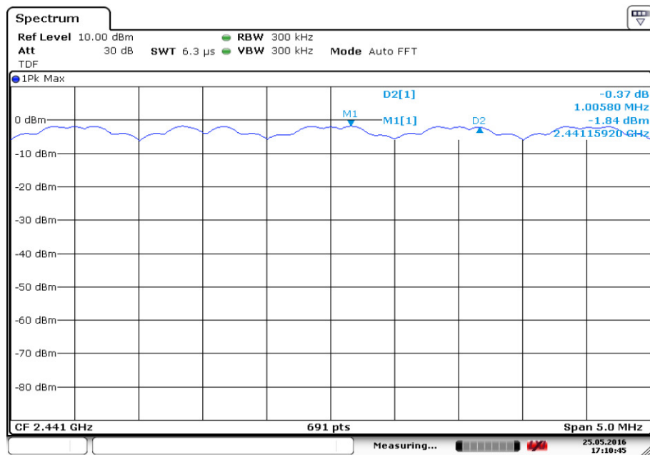
Fig.79. Carrier frequency separation measurement: \pi/4 DQPSK, Channel 39
