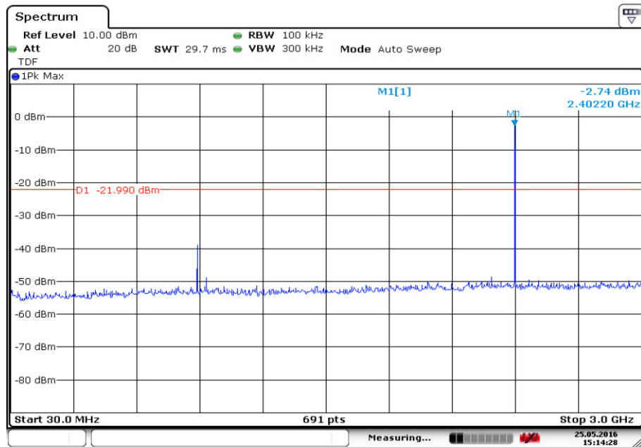
Fig.32. Conducted Spurious Emission (8DPSK, Ch0, 30 MHz-3 GHz)
