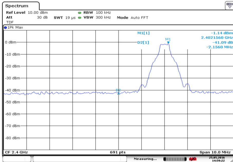
Fig.1. Frequency Band Edges: GFSK, Channel 0, Hopping Off
