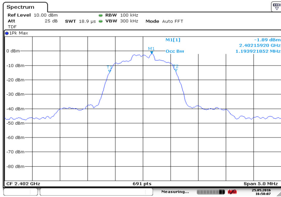
Fig.90. Occupied Bandwidth: \pi/4 DQPSK, Channel 0
