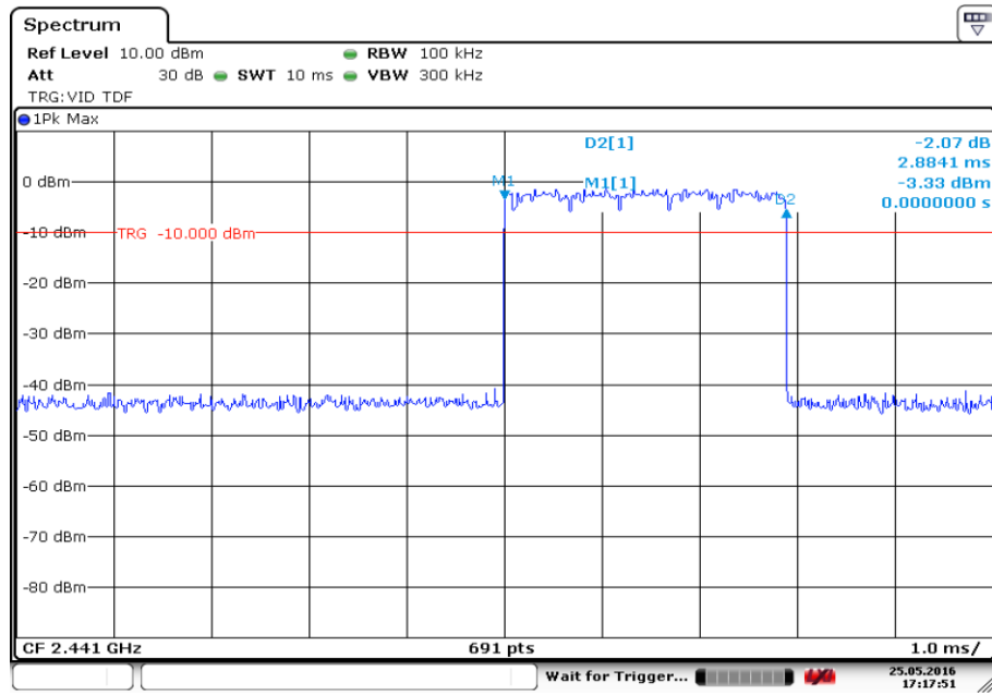
Fig.63. Time of occupancy (Dwell Time): Channel 39, Packet DH5
