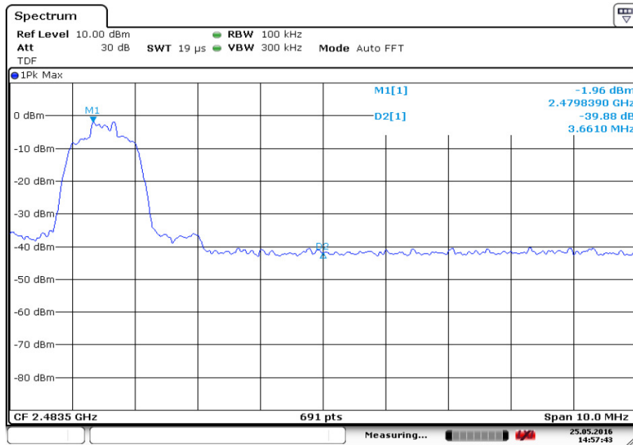
Fig.7. Frequency Band Edges: \pi/4 DQPSK, Channel 78, Hopping Off
