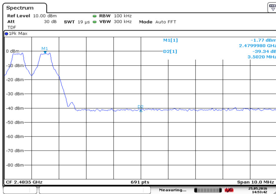
Fig.4. Frequency Band Edges: GFSK, Channel 78, Hopping On
