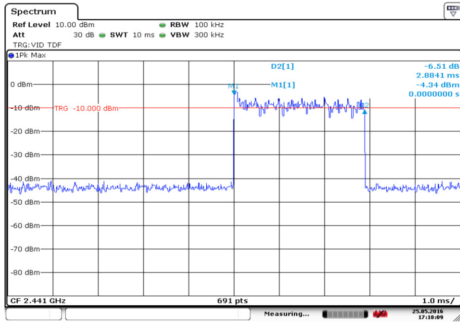
Fig.65. Time of occupancy (Dwell Time): Channel 39, Packet 2-DH5
