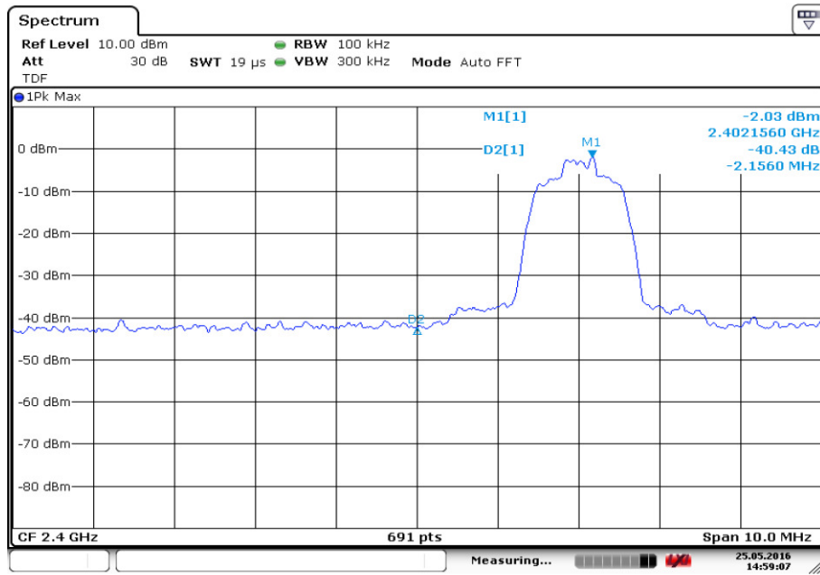
Fig.5. Frequency Band Edges: \pi/4 DQPSK, Channel 0, Hopping Off
