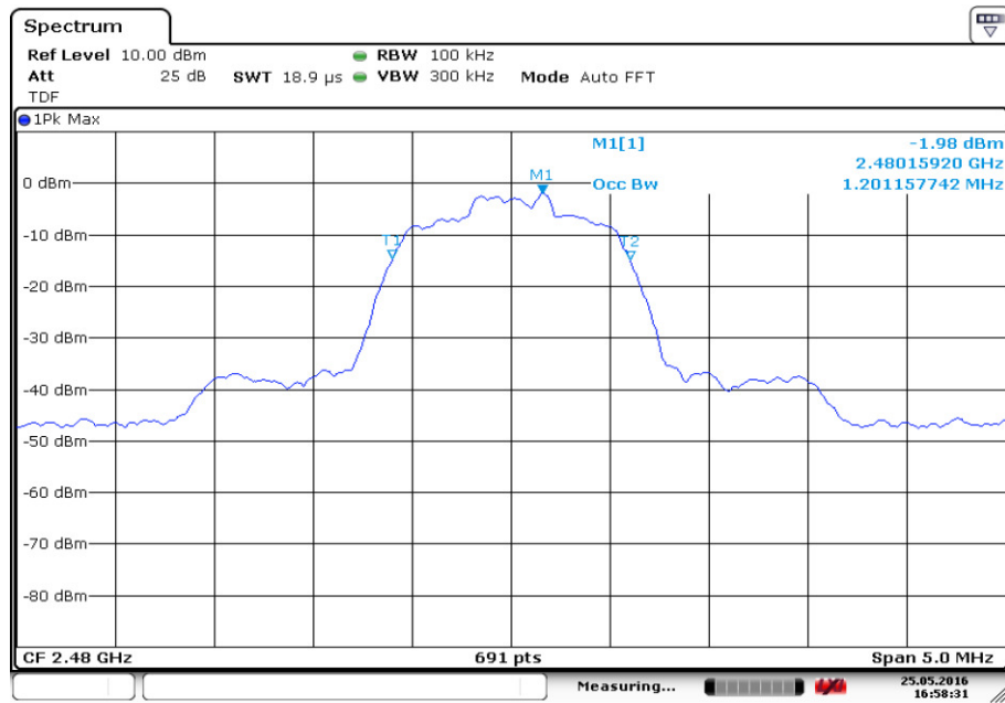
Fig.92. Occupied Bandwidth: \pi/4 DQPSK, Channel 78
