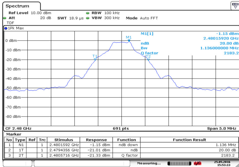
Fig.71. 20dB Bandwidth: GFSK, Channel 78
