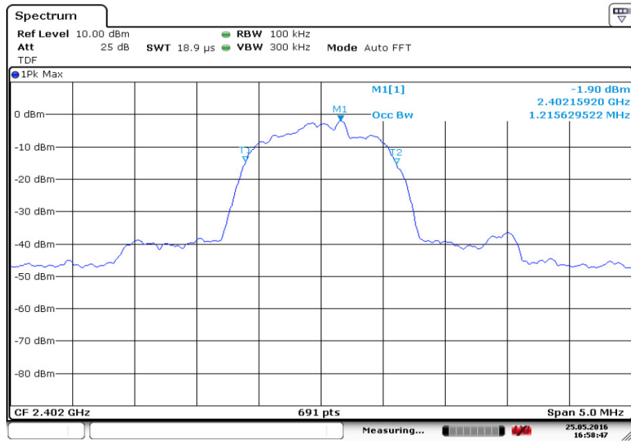
Fig.93. Occupied Bandwidth: 8DPSK, Channel 0
