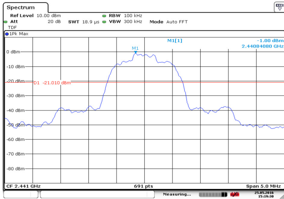
Fig.34. Conducted Spurious Emission (8DPSK, Ch39, 2.441GHz)
