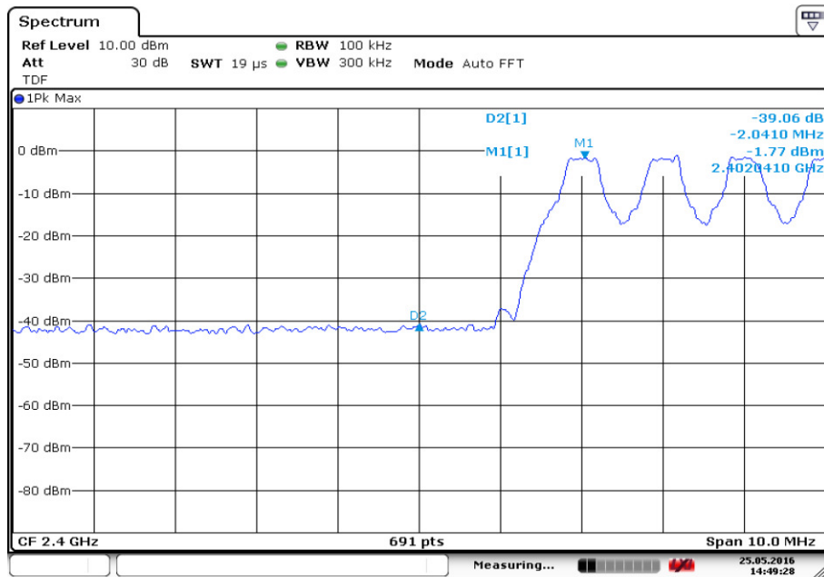
Fig.2. Frequency Band Edges: GFSK, Channel 0, Hopping On
