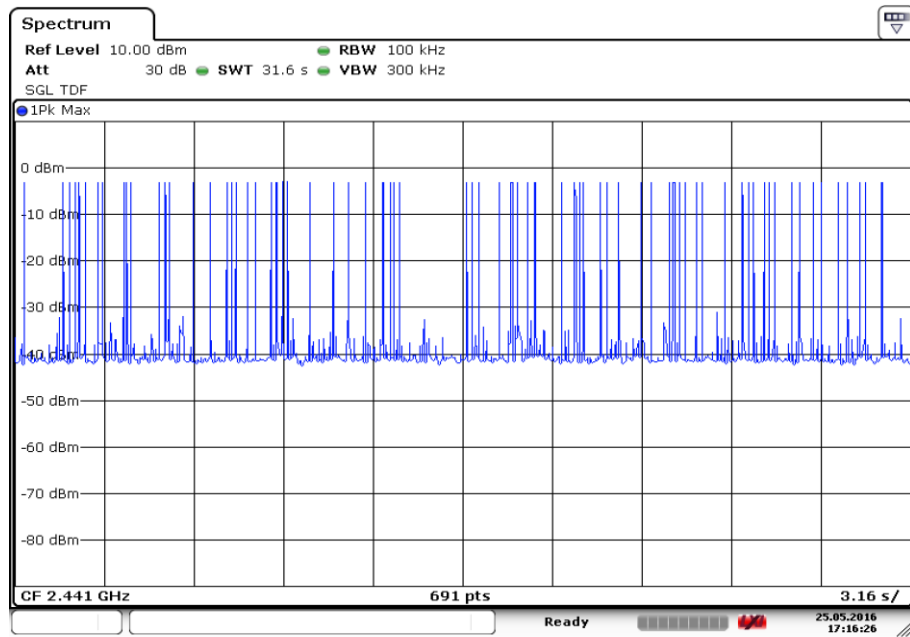
Fig.66. Number of Transmissions Measurement: Channel 39, Packet 2-DH5
