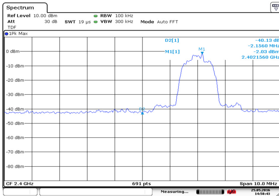
Fig.9. Frequency Band Edges: 8DPSK, Channel 0, Hopping Off
