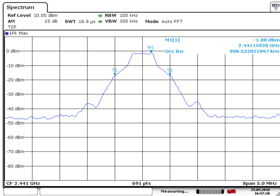
Fig.88. Occupied Bandwidth: GFSK, Channel 39
