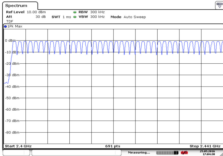
Fig.81. Number of hopping frequencies: GFSK, Channel 0 - 39
