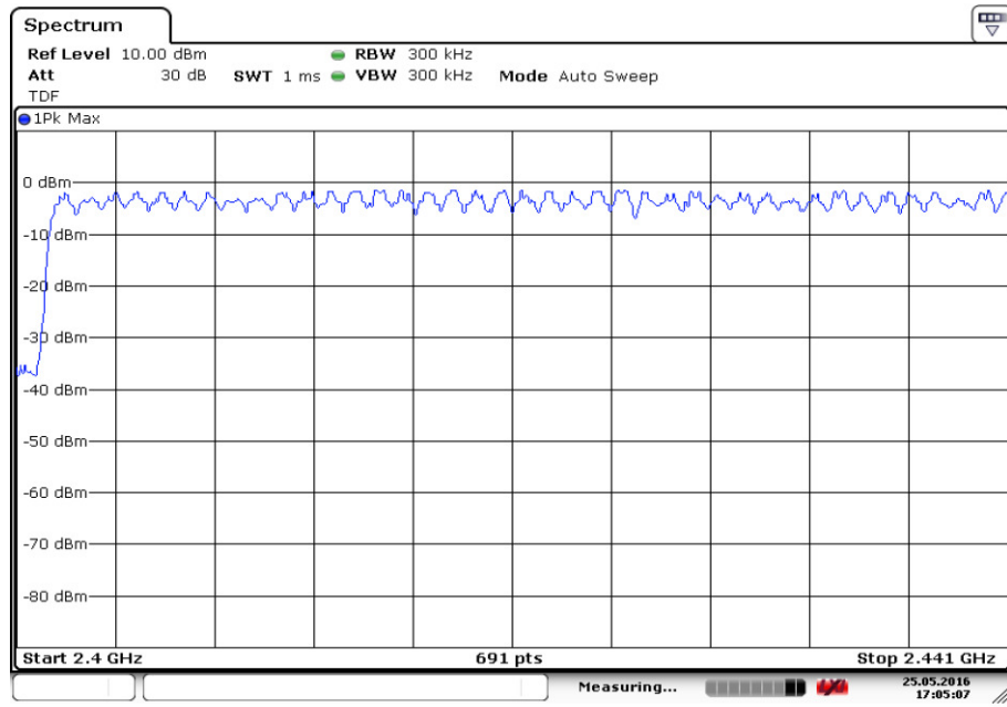
Fig.83. Number of hopping frequencies: \pi/4 DQPSK, Channel 0 - 39
