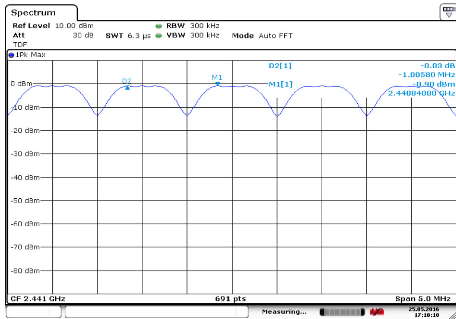
Fig.78. Carrier frequency separation measurement: GFSK, Channel 39
