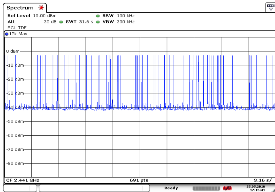
Fig.68. Number of Transmissions Measurement: Channel 39, Packet 3-DH5
