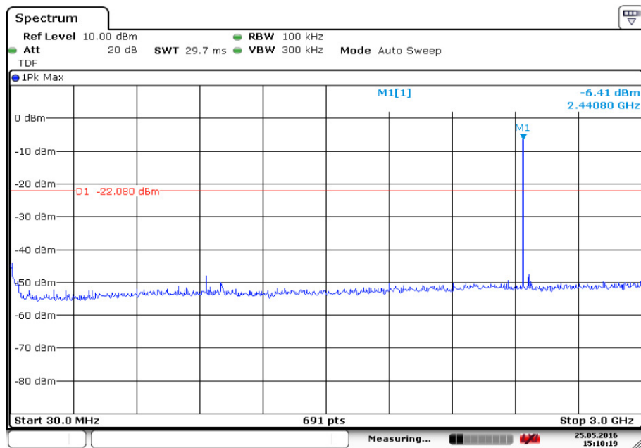
Fig.26. Conducted Spurious Emission ( \pi /4 DQPSK, Ch39, 30 MHz-3 GHz)
