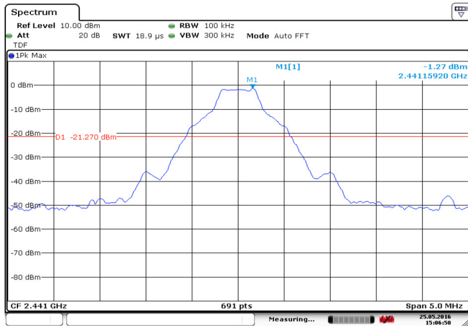
Fig.16. Conducted Spurious Emission (GFSK, Ch39, 2.441GHz)
