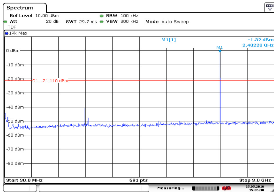
Fig.14. Conducted Spurious Emission (GFSK, Ch0, 30 MHz-3 GHz)
