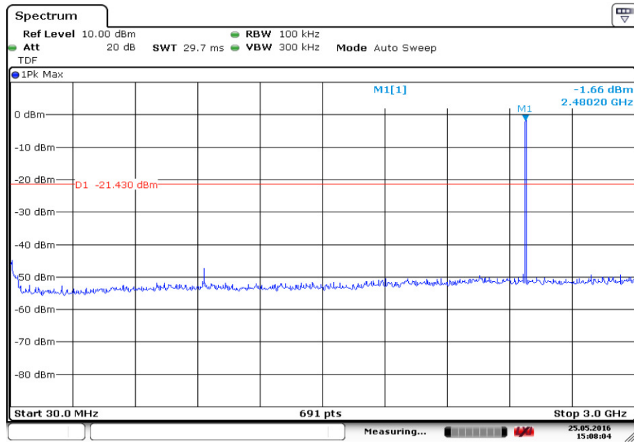
Fig.20. Conducted Spurious Emission (GFSK, Ch78, 30 MHz-3 GHz)
