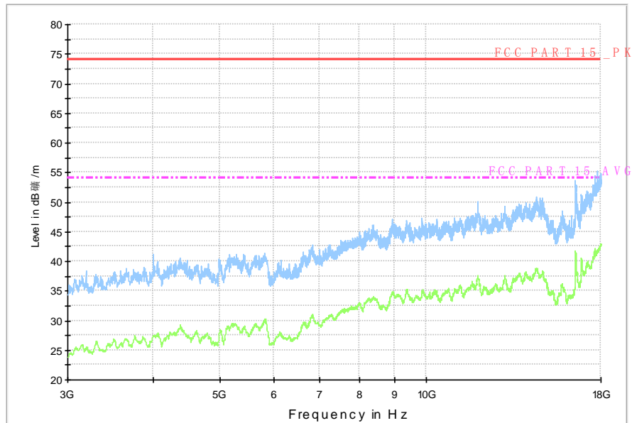
Normal RE_3G-18GHz
