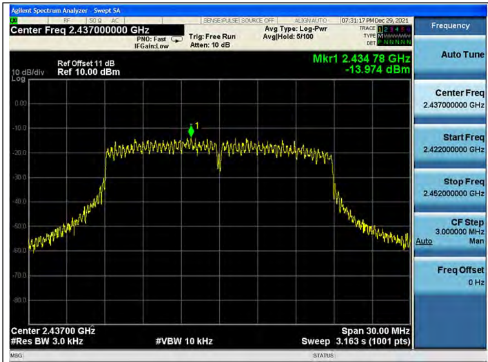
(Channel 6, 802.11n (HT20), ANT1)
