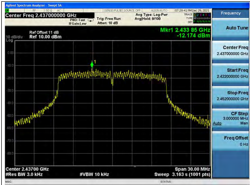
(Channel 6, 802.11g, ANT1)
