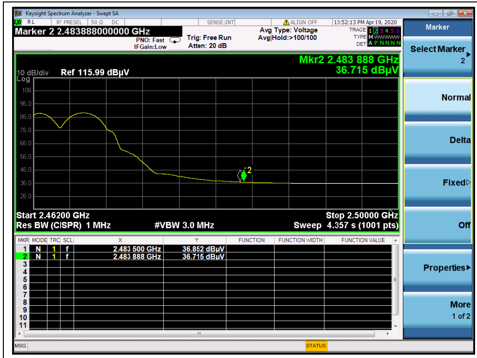
(AVG, Channel = 11, 802.11g)
