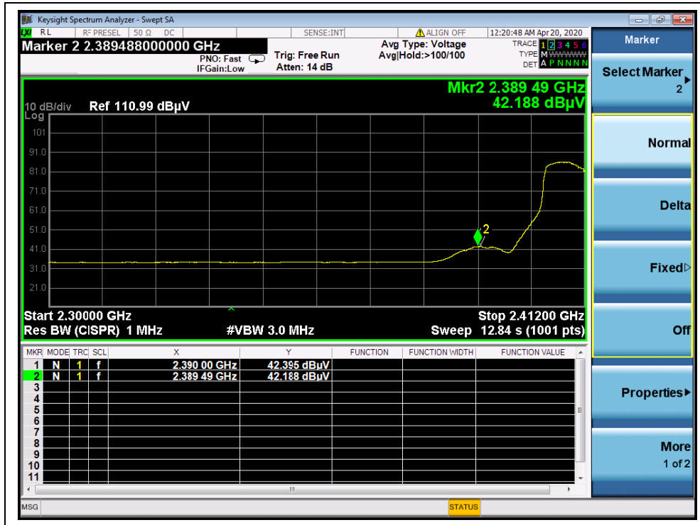
(AVG, Channel = 3, 802.11n(HT40))
