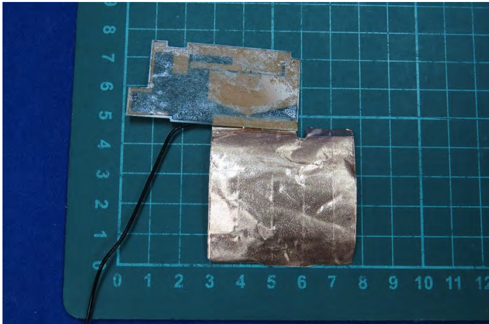
(29) EUT Photo_WWAN_SPEED/F-0G-MA-6001-001-00(Main)
