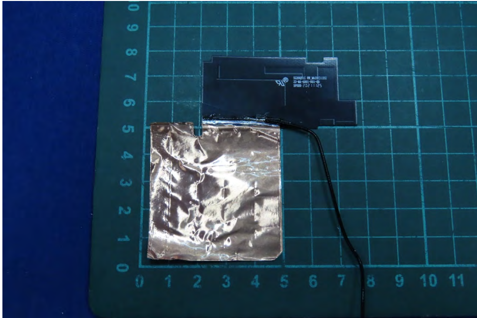
(28) EUT Photo_WWAN_SPEED/F-0G-MA-6001-001-00(Main)
