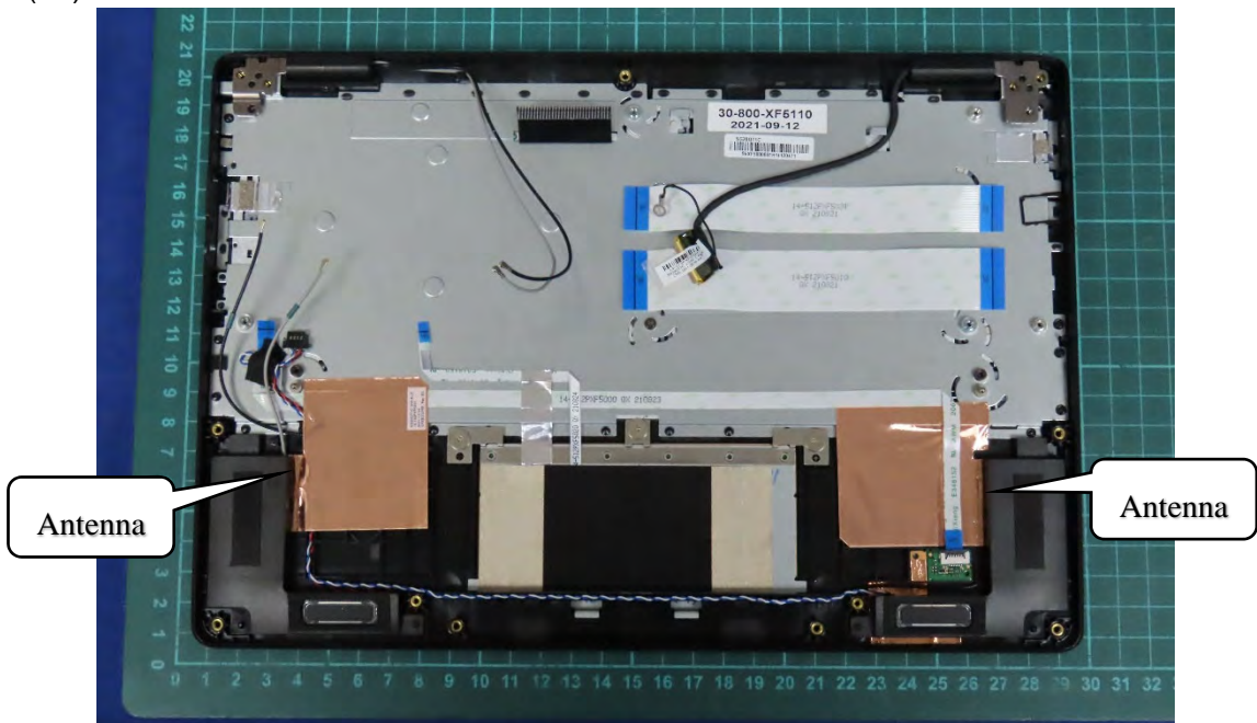
(26) EUT Photo
