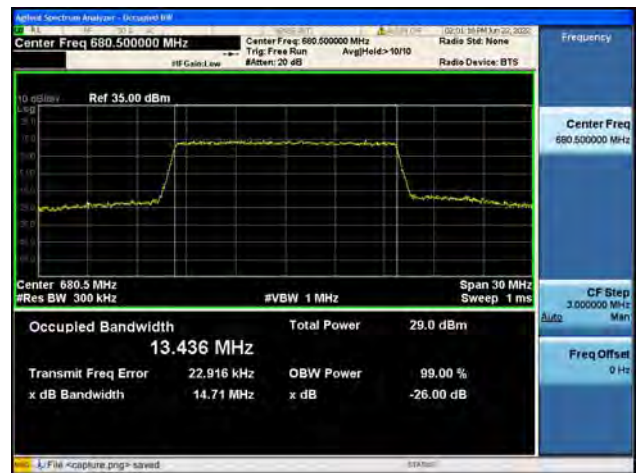
B71 / 15MHz / 64QAM/ Mid CH
